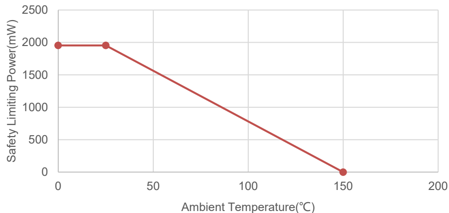
Figure 7.1 NSI3600D Thermal Derating Curve, Dependence of Safety Limiting Values with Case Temperature per DIN VDE V 0884-11
