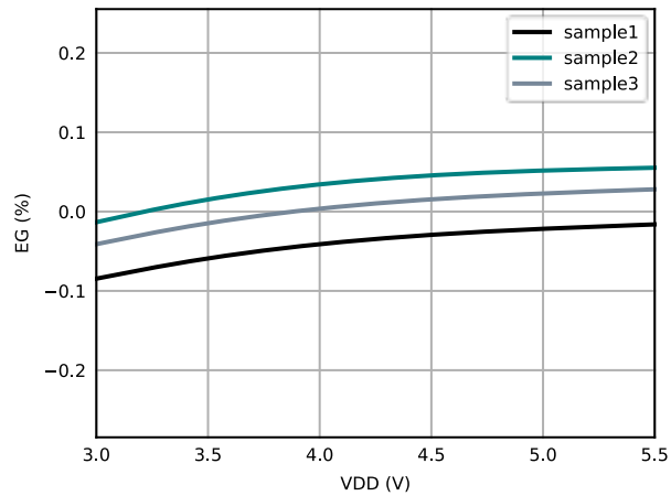
Figure 6.10 Gain Error vs Supply Voltage
