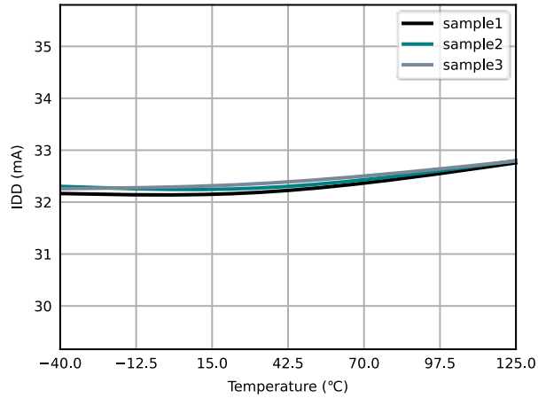
Figure 6.24 Input Supply Current vs Temperature ( I_E=1\text{mA} )
