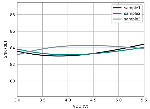
Figure 6.15 Signal to Noise Ratio vs Supply Voltage
