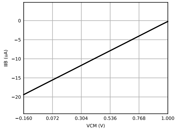
Figure 6.4 Input Bias Current vs Common-Mode Input Voltage
