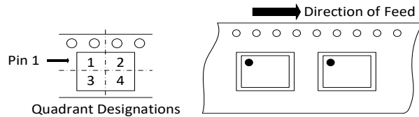
Figure 13.2 Tape Information of SOP16(300mil)
