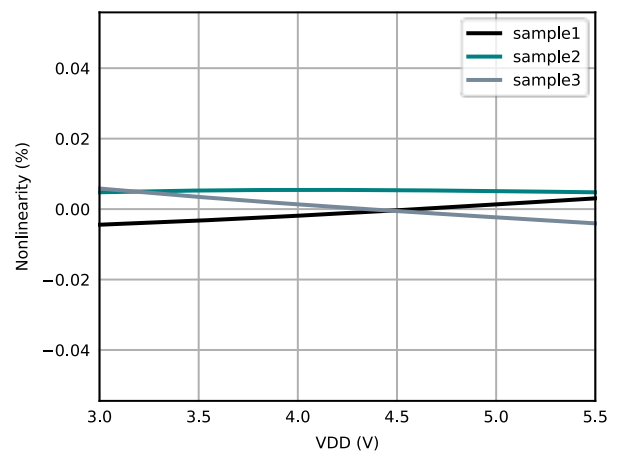
Figure 6.13 Nonlinearity vs Supply Voltage
