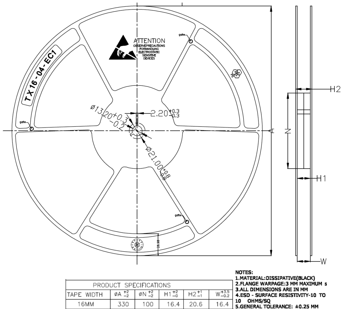
Figure 13.1 Reel Information
