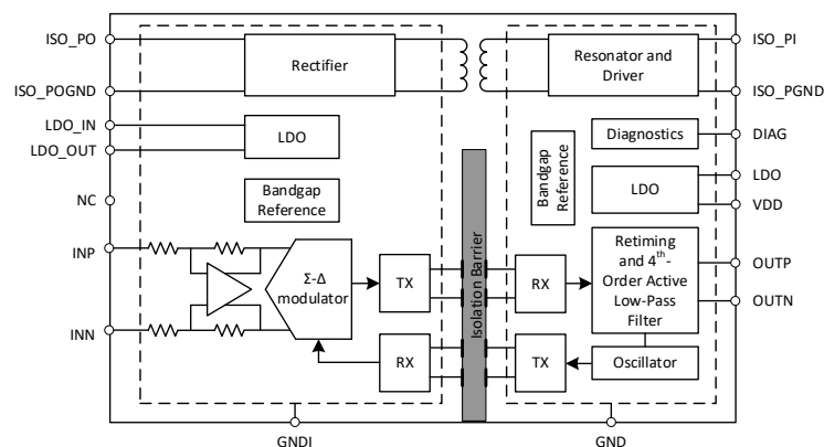
Figure 1. Function Block Diagram of NSI3600D
