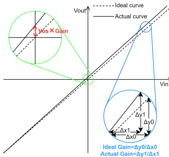
Figure 8.2 V_{\text{os}} and EG diagram
