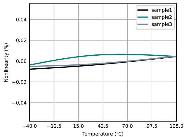
Figure 6.12 Nonlinearity vs Temperature
