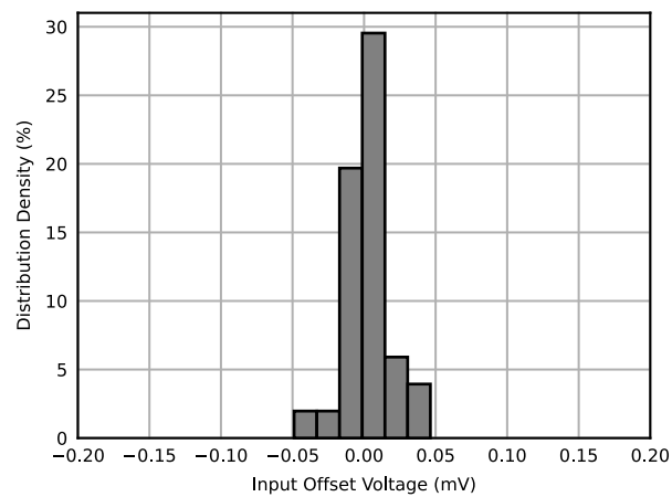
Figure 6.8 Input Offset Voltage Distribution (1)
