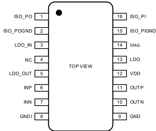
Figure 1.1 NSI3600D Package
