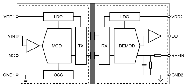
Figure 1. NSI1611S50-Q1 Block Diagram
