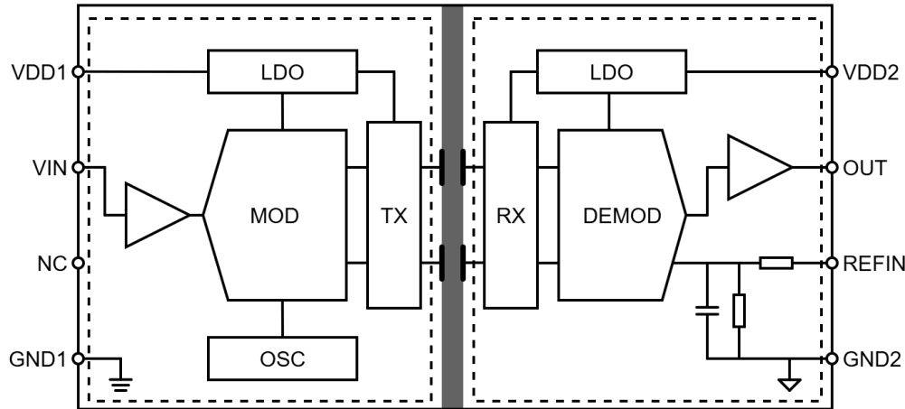
Figure 8.1 Function Block Diagram of NSI1611S50-Q1
