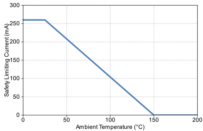
Figure 7.1 NSI1611S50-Q1 Thermal Derating Curve, Dependence of Safety Limiting Values with Case Temperature per DIN VDE V 0884-11
