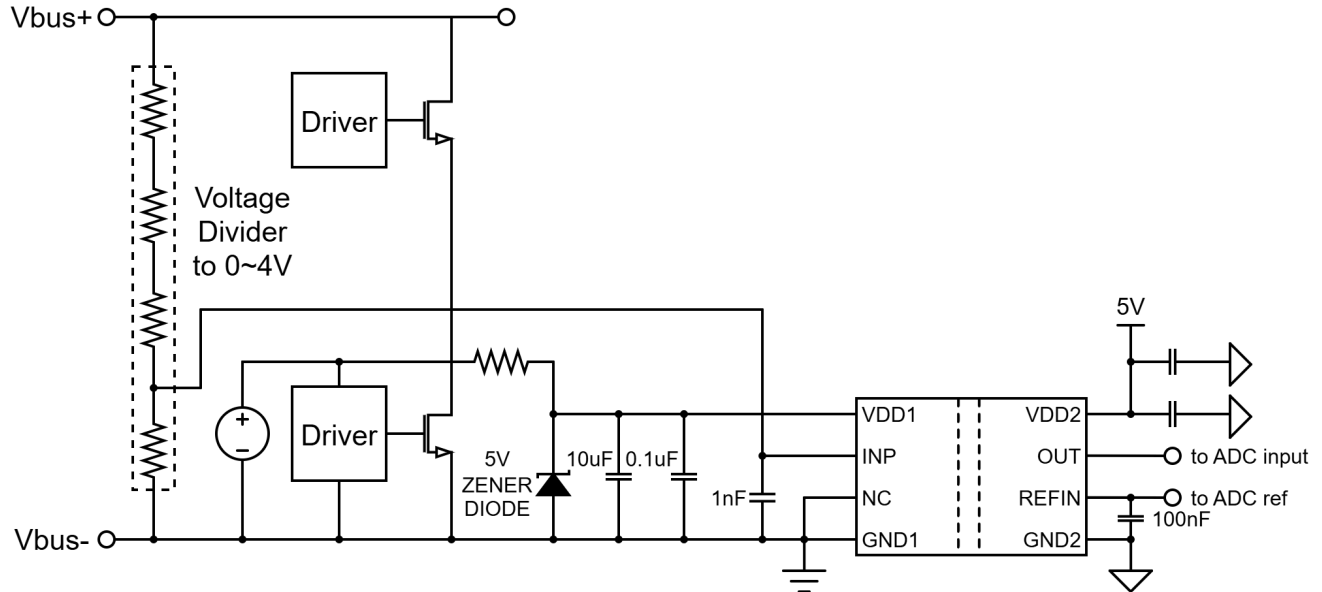
Figure 9.1 Typical Application Diagram of NSI1611S50-Q1
