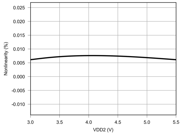
Figure 6.13 Nonlinearity vs VDD2
