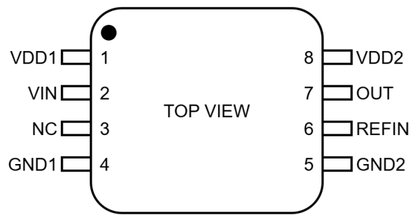
Figure 1.1 NSI1611S50-Q1 Package(Not to scale)
