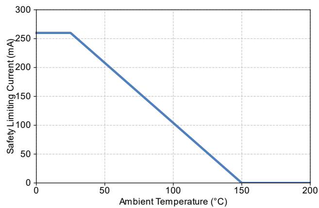
Figure 7.1 NSI1611S33-Q1 Thermal Derating Curve, Dependence of Safety Limiting Values with Case Temperature per DIN VDE V 0884-11
