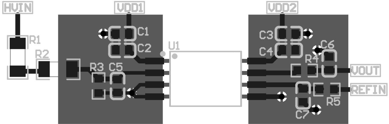
Figure 9.4 PCB layout example of NSI1611S33-Q1
