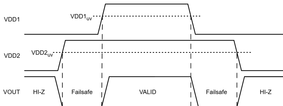
Figure 8.4 Waveform of NSI1611S33-Q1 when power fails
