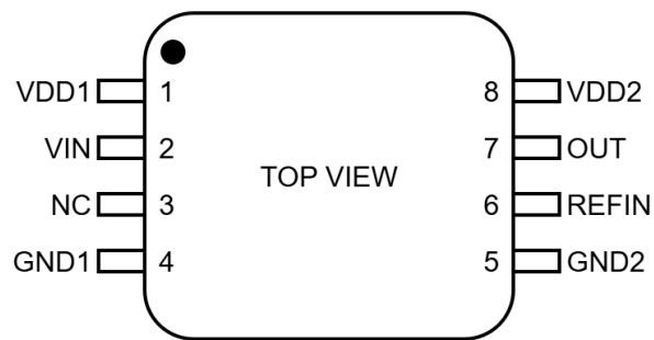
Figure 1.1 NSI1611S33-Q1 Package(Not to scale)
