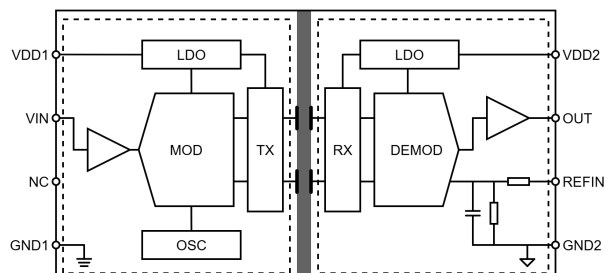
Figure 1. NSI1611S33-Q1 Block Diagram
