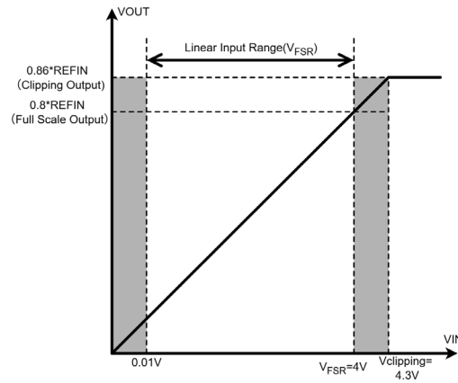
Figure 8.2 Input to Output Transfer Curve of the NSI1611S33
