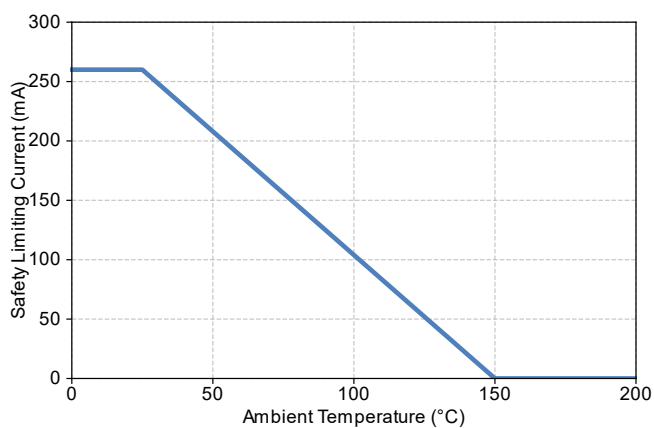
Figure 7.1 NSI1611S33 Thermal Derating Curve, Dependence of Safety Limiting Values with Case Temperature per DIN VDE V 0884-11
