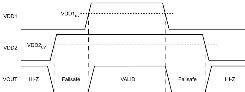
Figure 8.4 Waveform of NSI1611S33 when power fails
