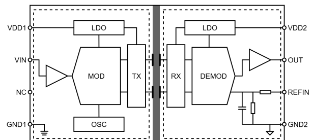
Figure 1. NSI1611S33 Block Diagram
