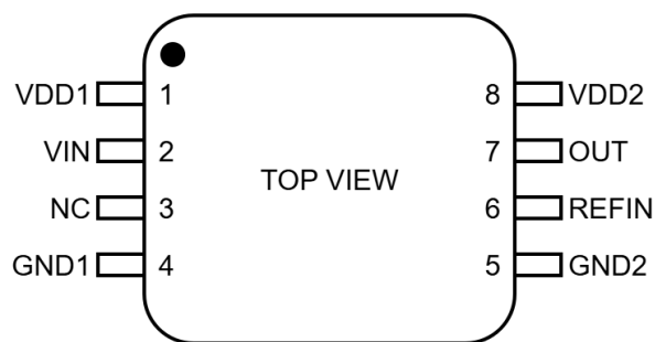
Figure 1.1 NSI1611S33 Package(Not to scale)
