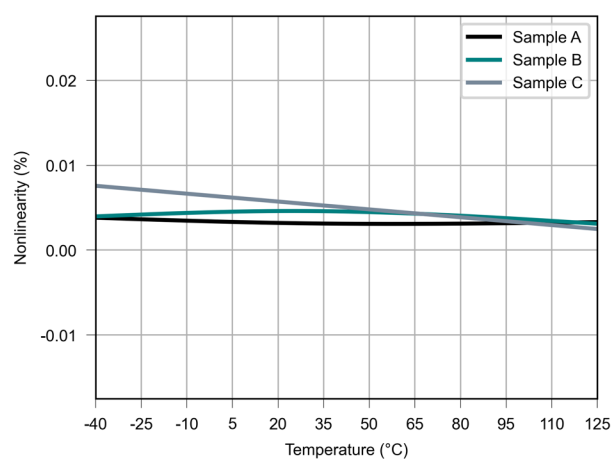
Figure 6.29 Nonlinearity vs Temperature
