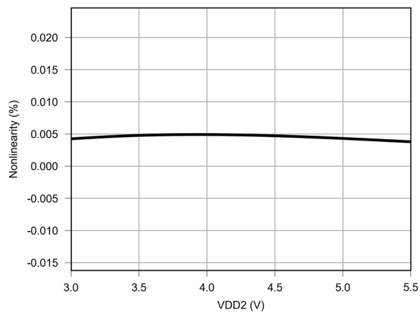
Figure 6.28 Nonlinearity vs VDD2
