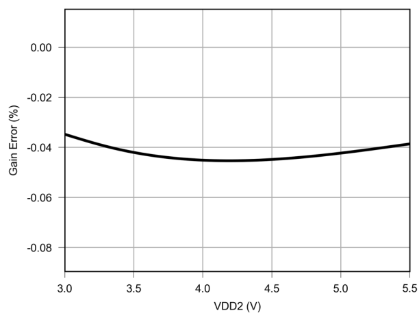
Figure 6.22 EG vs VDD2
