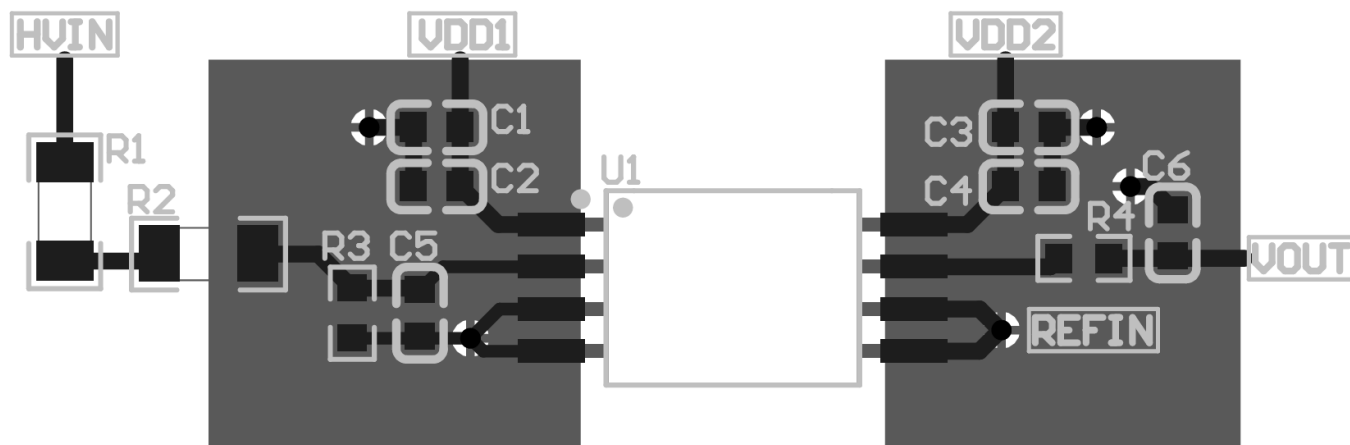
Figure 9.4 PCB layout example of NSI1611S0x-Q1
