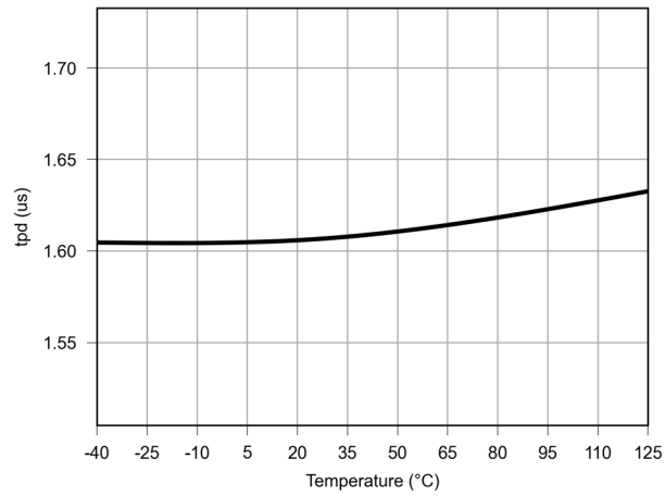
Figure 6.32 Propagation Delay vs Teperature
