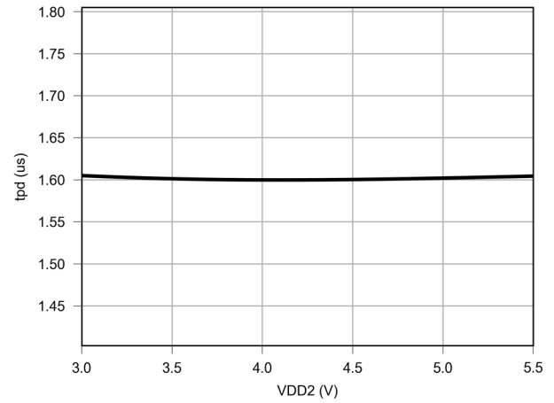
Figure 6.31 Propagation Delay vs VDD2
