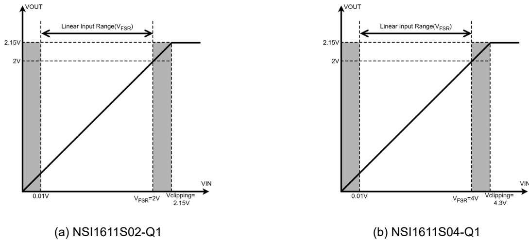
Figure 8.2 Input to Output Transfer Curve of the NSI1611S0x-Q1
