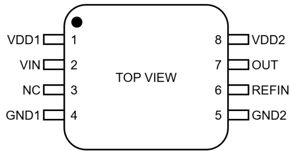
Figure 1.1 NSI1611S0x-Q1 Package(Not to scale)
