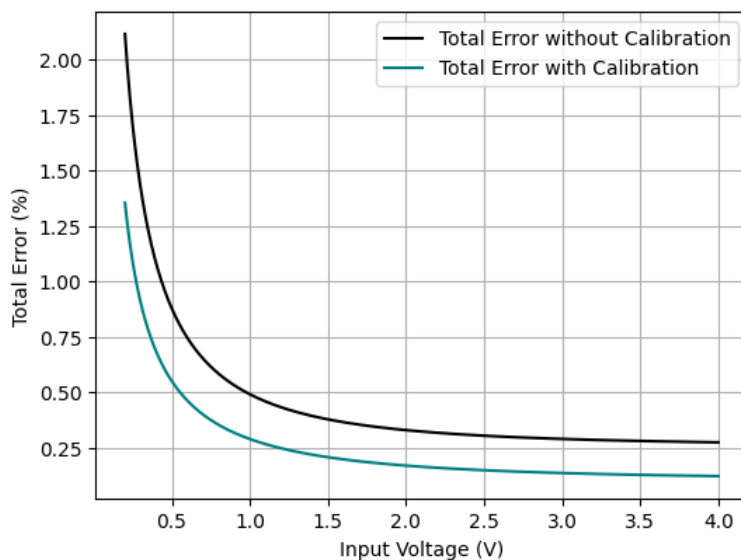
Figure 9.3 Total Error Over -40°C to 85°C vs Input Voltage
