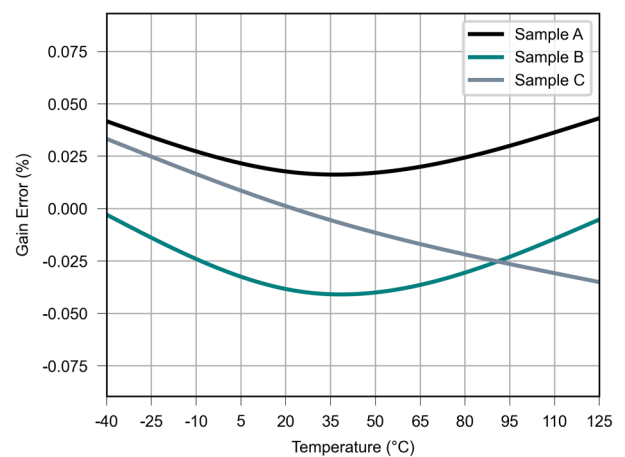
Figure 6.23 EG vs Temperature
