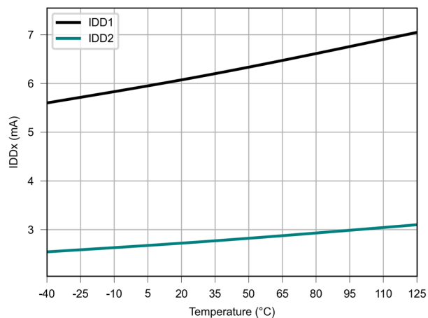
Figure 6.26 IDDX vs Temperature
