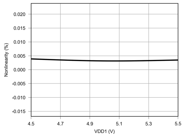
Figure 6.27 Nonlinearity vs VDD1
