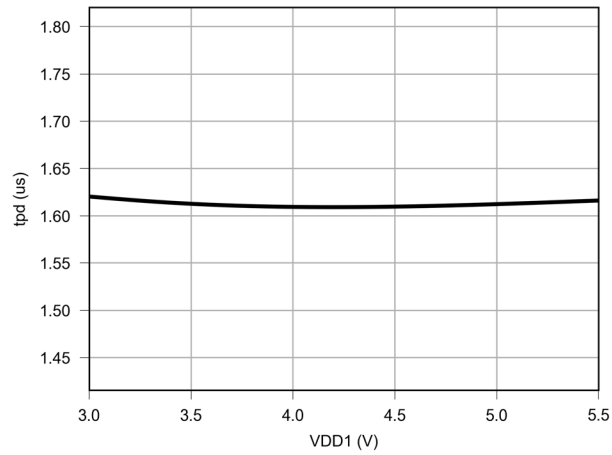
Figure 6.30 Propagation Delay vs VDD1
