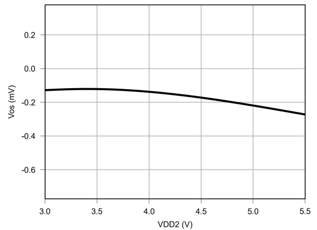
Figure 6.19 Vos vs VDD2
