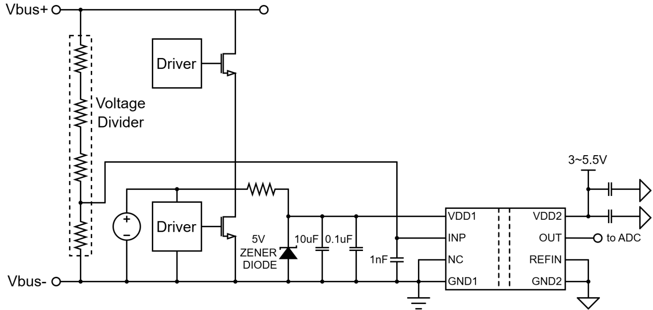
Figure 9.1 Typical Application Diagram of NSI1611S0x-Q1
