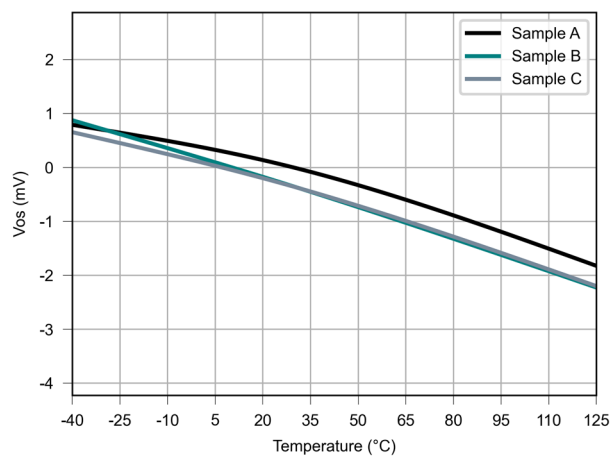
Figure 6.20 Vos vs Temperature
