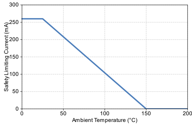
Figure 7.1 NSI1611S0x-Q1 Thermal Derating Curve, Dependence of Safety Limiting Values with Case Temperature per DIN VDE V 0884-11
