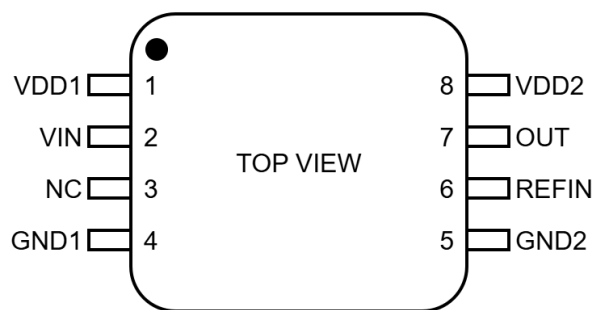
Figure 1.1 NSI1611S0x Package(Not to scale)
