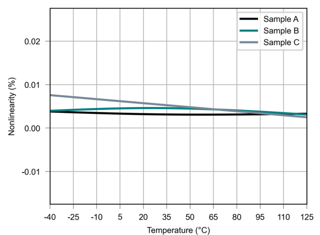
Figure 6.29 Nonlinearity vs Temperature
