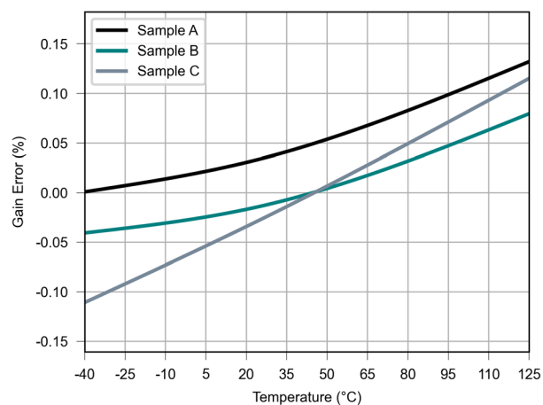
Figure 6.8 EG vs Temperature
