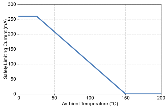
Figure 7.1 NSI1611S0x Thermal Derating Curve, Dependence of Safety Limiting Values with Case Temperature per DIN VDE V 0884-11
