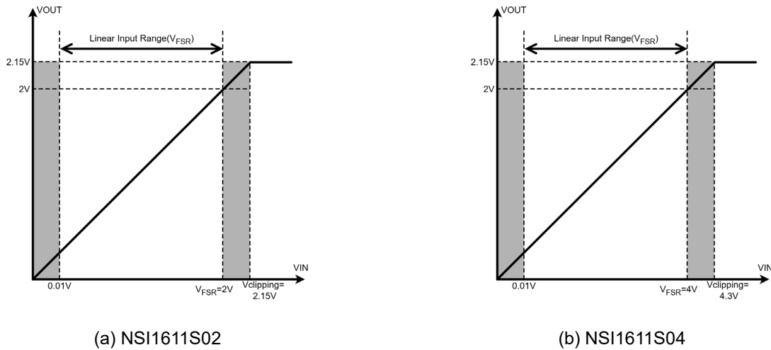
Figure 8.2 Input to Output Transfer Curve of the NSI1611S0x
