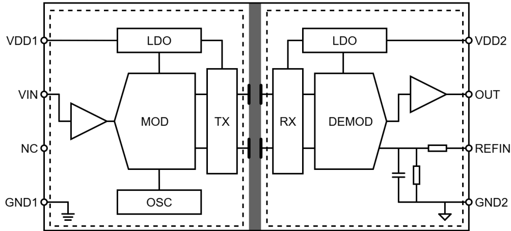
Figure 8.1 Function Block Diagram of NSI1611S0x
