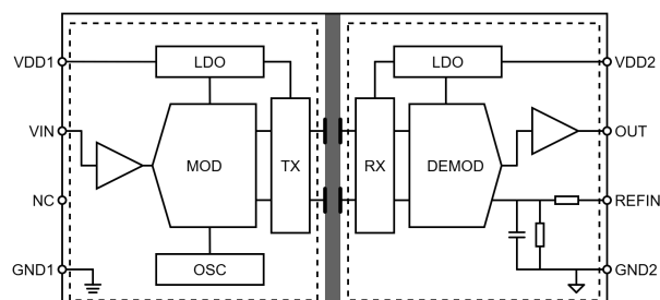
Figure 1. NSI1611S0x Block Diagram
