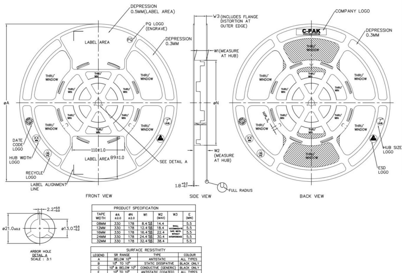
Figure 13.1 Tape Information
