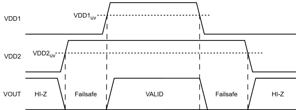
Figure 8.4 Waveform of NSI1611S0x when power fails
