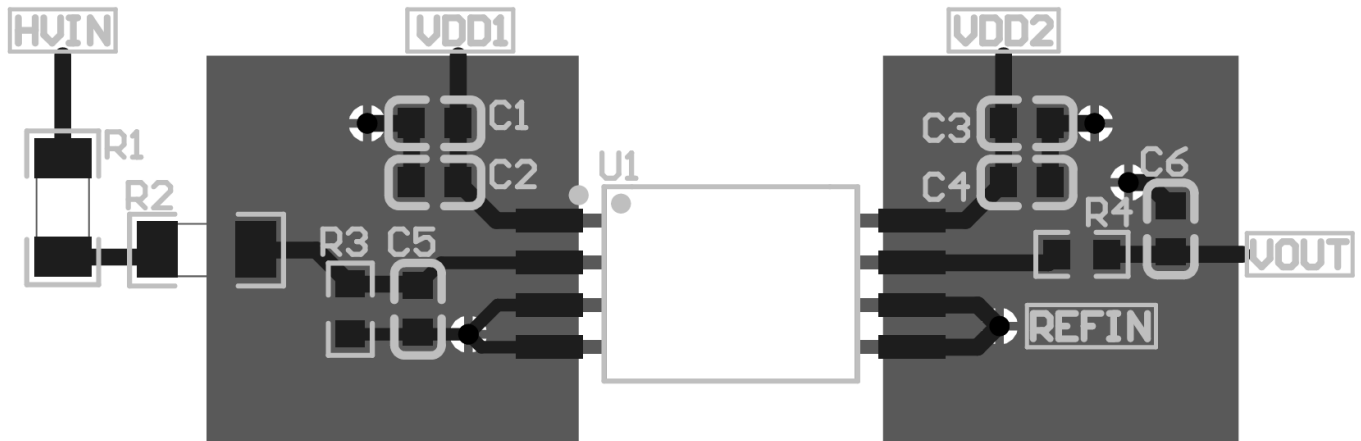
Figure 9.4 PCB layout example of NSI1611S0x
