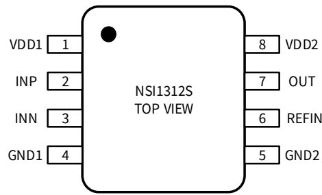
Figure 1.2 NSI1312S Package
