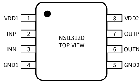
Figure 1.1 NSI1312D Package
