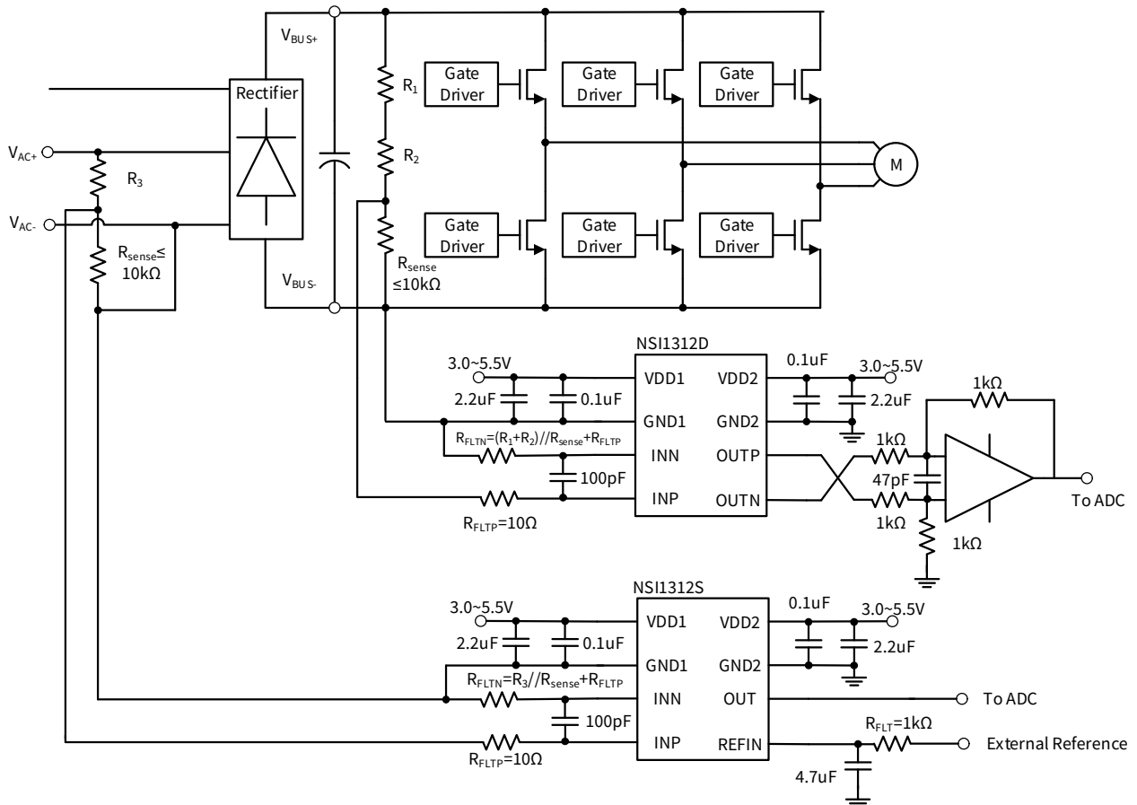
Figure 9.1 Typical application circuit in voltage sensing
