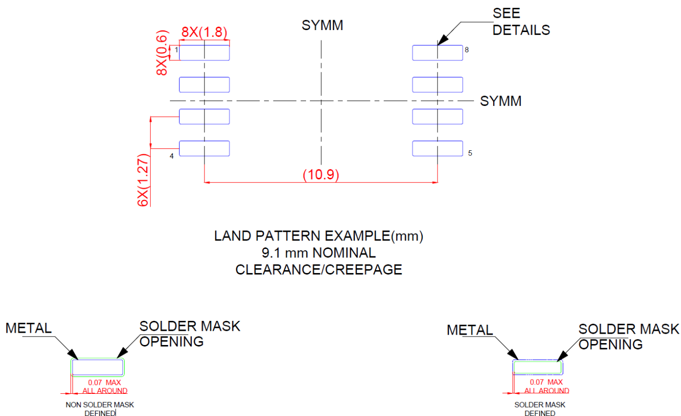
Figure 10.2 SOW8 Package Board Layout Example
