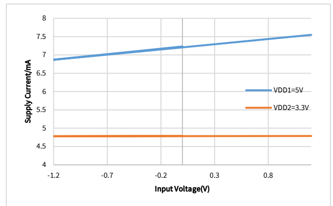
Figure 6.16 Supply Current vs Input Voltage
