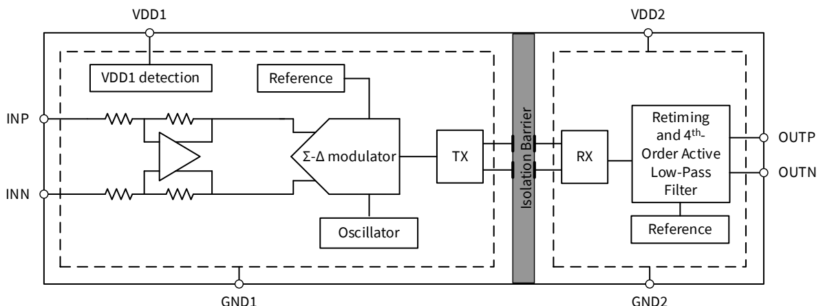
Figure 8.1 Function Block Diagram of Differential Output Version
