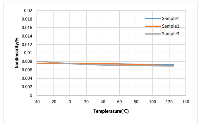
Figure 6.3 Nonlinearity vs Temperature
