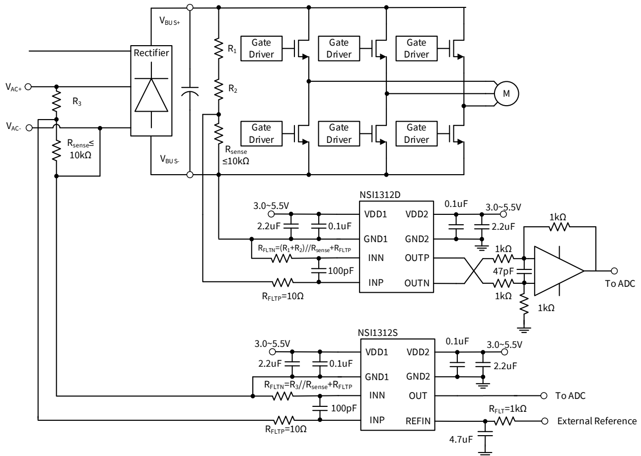
Figure 9.1 Typical application circuit in voltage sensing
