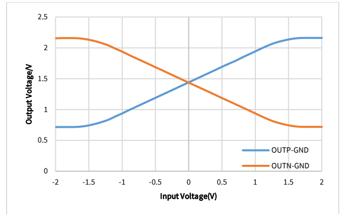
Figure 6.12 Output Voltage vs Input Voltage (NSI1312D)
