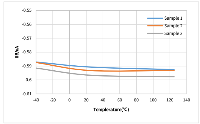
Figure 6.4 Input Bias Current vs Temperature
