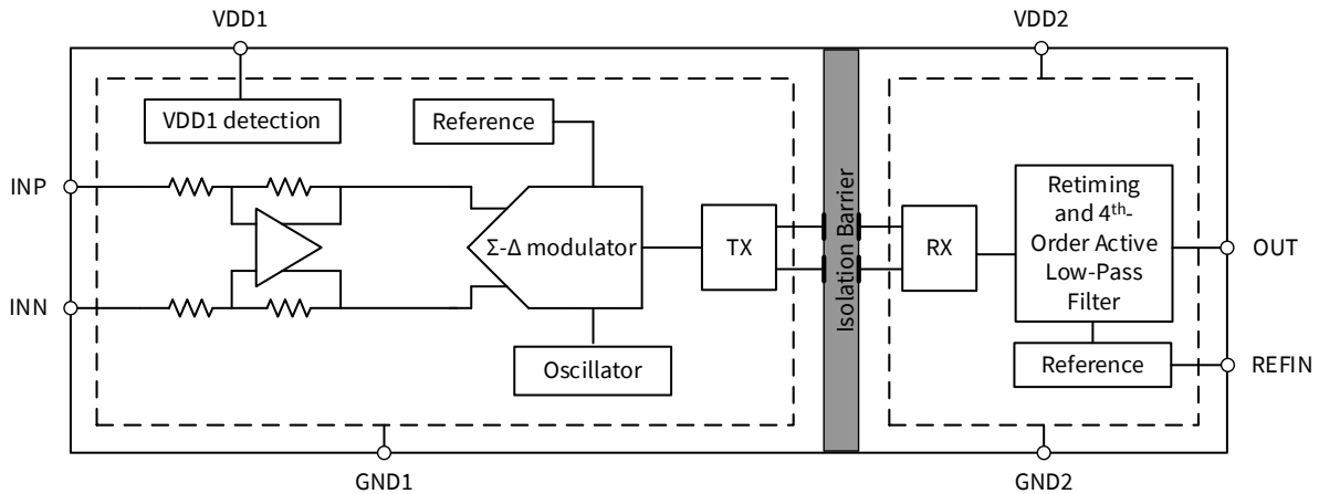
Figure 8.2 Function Block Diagram of Single-ended Output Version
