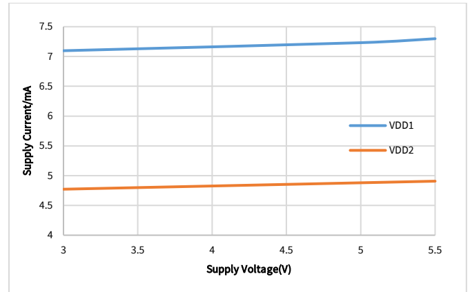
Figure 6.18 Supply Current vs Supply Voltage
