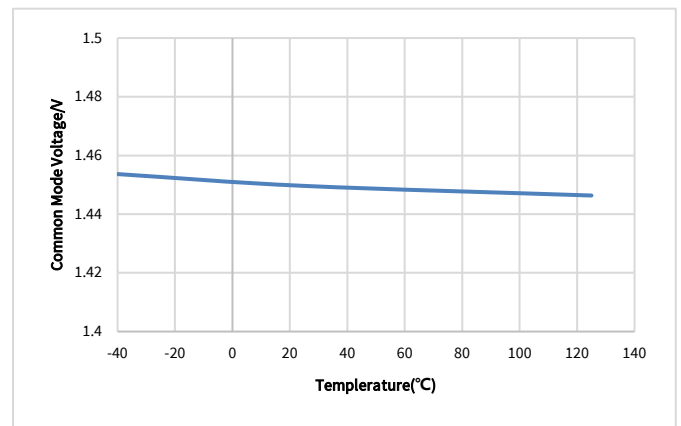
Figure 6.14 Output Common-Mode Voltage vs Temperature (NSI1312D)
