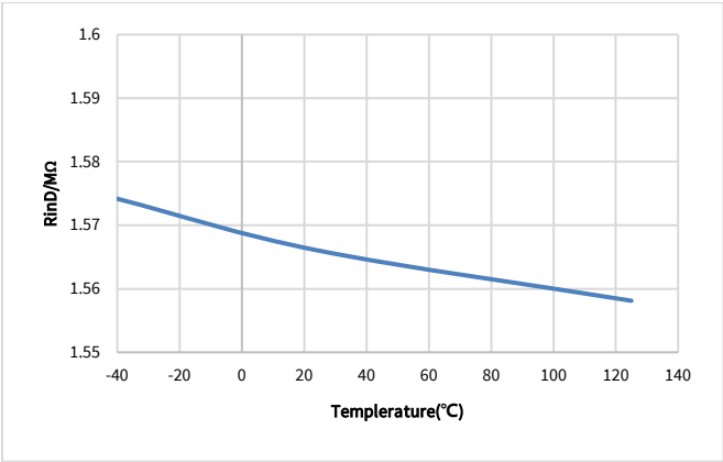
Figure 6.6 Differential Input Resistance vs Temperature
