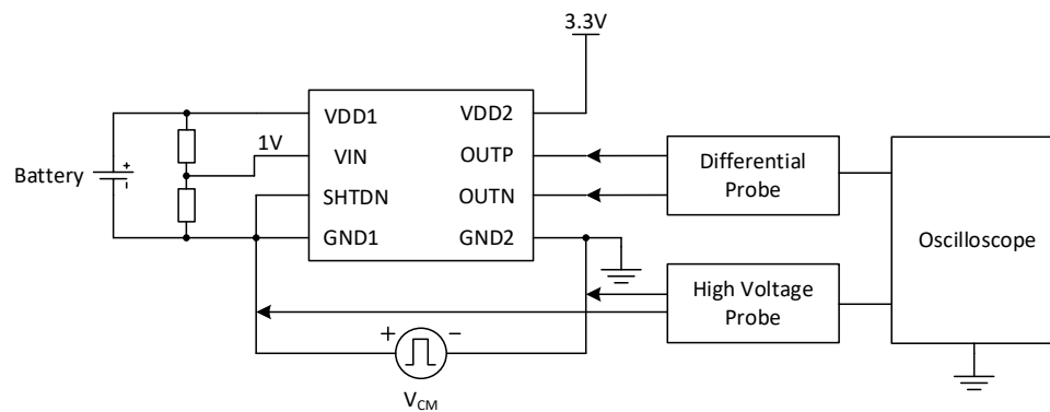
Figure 5.12 Common-Mode Transient Immunity Test Circuit
