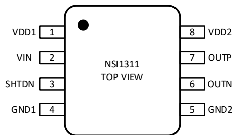
Figure 1.1 NSI1311 Package
