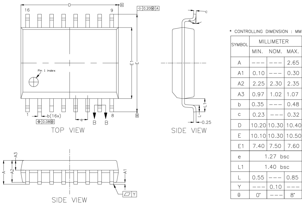
Figure 10.3 SOW16 package shape and dimension in millimeters
