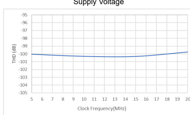
Figure 6.13 Total Harmonic Distortion vs Clock Frequency
