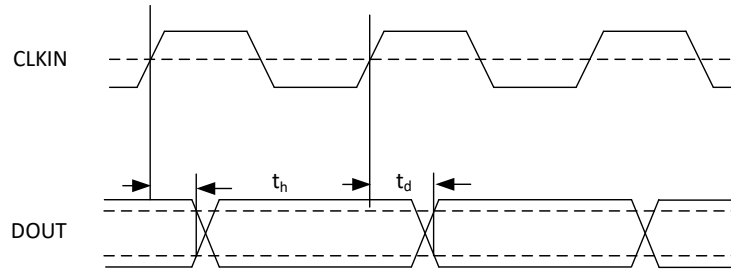
Figure 6.1 Digital Input and Output Timing
