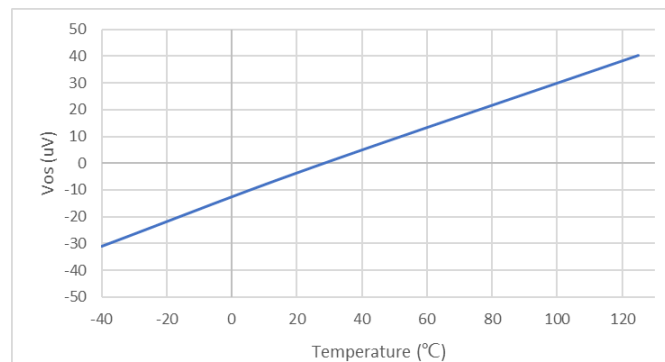
Figure 6.5 Input Offset Voltage vs Temperature
