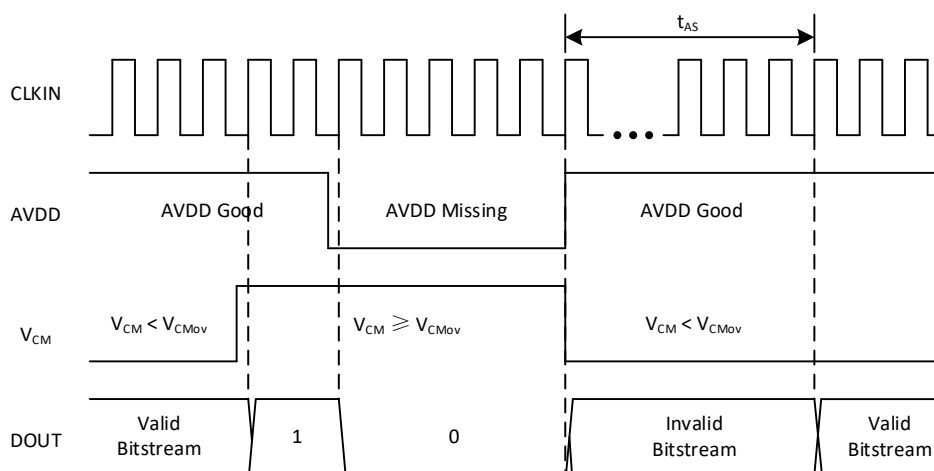
Figure 8.2 Fail-safe output
