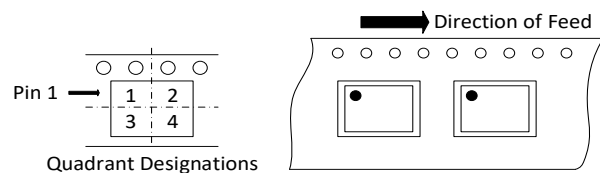
Figure 13.3 Tape Information of SOP16(300mil)
