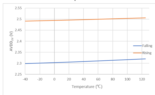
Figure 6.21 Analog Side Under-Voltage Detection Level vs Temperature
