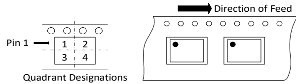
Figure 13.2 Tape Information of SOP8(300mil)
