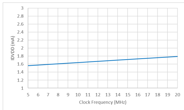
Figure 6.25 Digital Side Supply Current vs Clock Frequency
