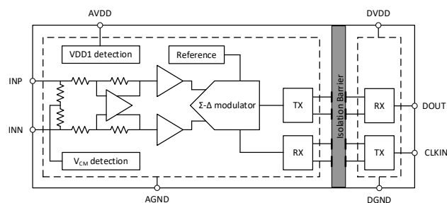
Figure 1. NSI1306C Block Diagram
