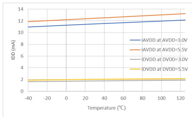
Figure 6.26 Supply Current vs Temperature
