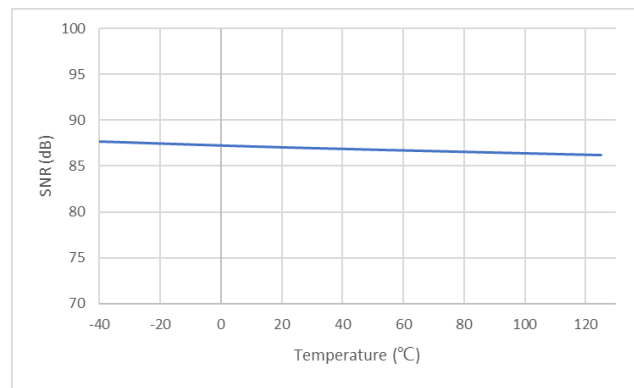
Figure 6.11 Signal-to-Noise Ratio vs Temperature
