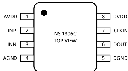
Figure 1.1 NSI1306C Package (SOP8(300mil))
