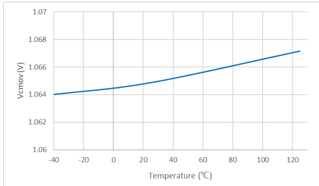
Figure 6.2 Common-Mode Overvoltage Detection Level vs Temperature
