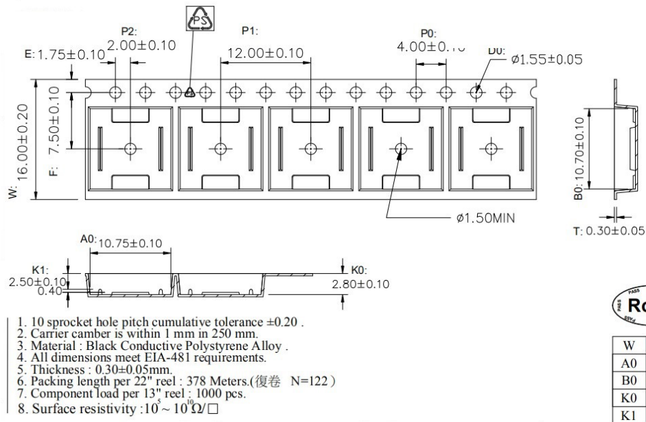
Figure 13.2 Tape Information of SOP8(300mil)
