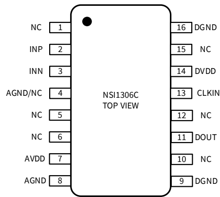
Figure 1.2 NSI1306C Package (SOP16(300mil))
