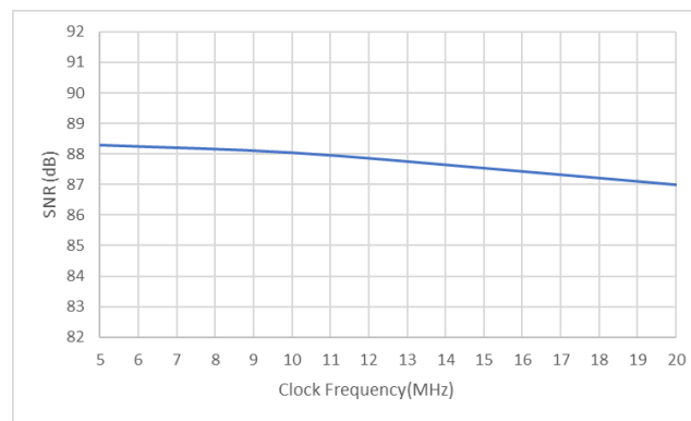
Figure 6.10 Signal-to-Noise Ratio vs Clock Frequency
