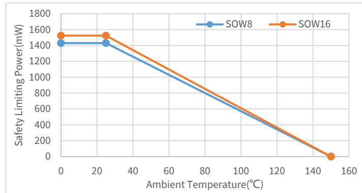
Figure 7.1 NSI1306C Thermal Derating Curve, Dependence of Safety Limiting Values with Case Temperature per DIN VDE V 0884-17
