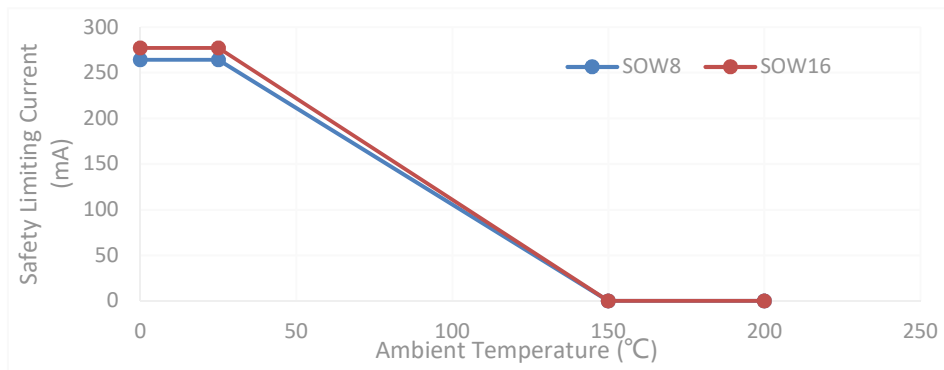
Figure 6.1 NSi1306C Thermal Derating Curve, Dependence of Safety Limiting Values with Case Temperature per DIN VDE V 0884-11
