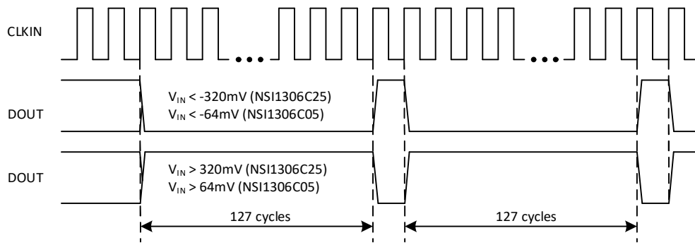
Figure 7.3 Overrange output
