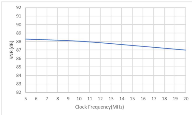
Figure 5.10 Signal-to-Noise Ratio vs Clock Frequency
