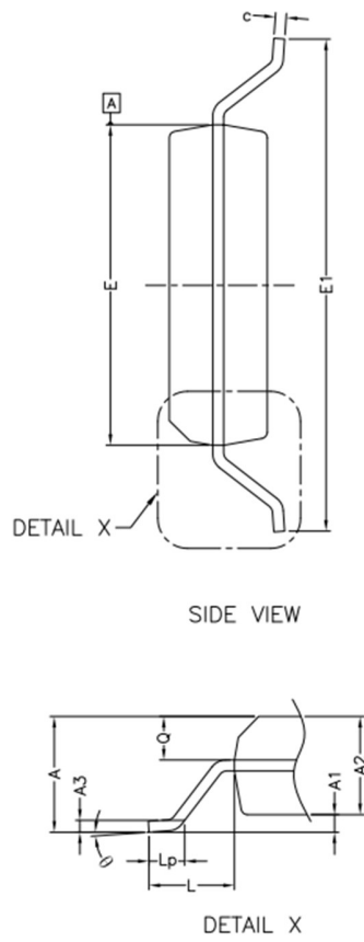
Figure 9.1 SOW8 Package Shape and Dimension in millimeters
