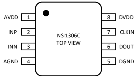
Figure 1.1 NSi1306C Package (SOP8(300mil))
