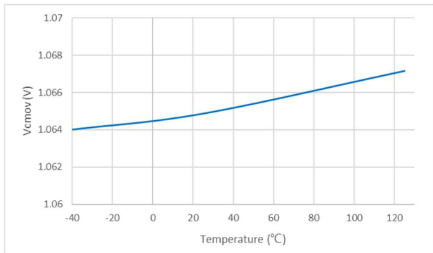
Figure 5.2 Common-Mode Overvoltage Detection Level vs Temperature
