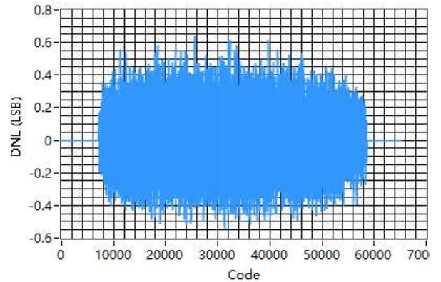
Figure 5.27 Typical Differential Nonlinearity
