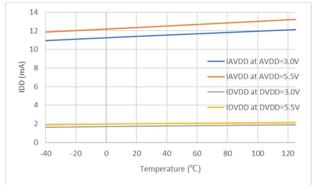
Figure 5.26 Supply Current vs Temperature
