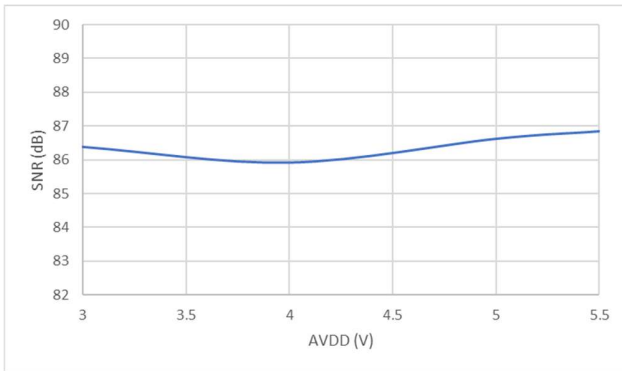
Figure 5.9 Signal-to-Noise Ratio vs Analog Side Supply Voltage
