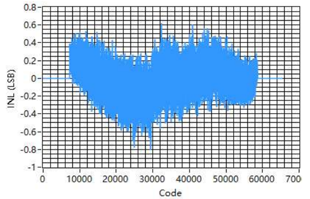
Figure 5.28 Typical Integral Nonlinearity
