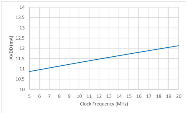
Figure 5.23 Analog Side Supply Current vs Clock Frequency
