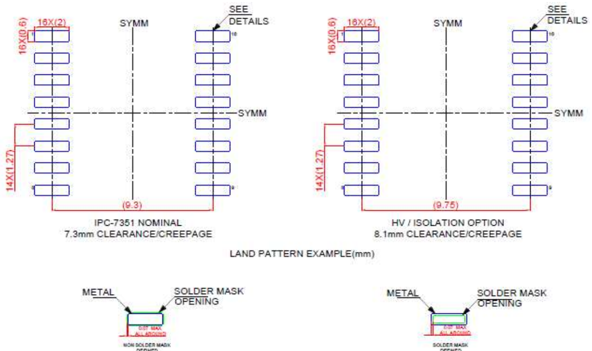
Figure 9.4 SOW16 Package Board Layout Example
