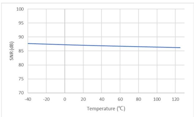
Figure 5.11 Signal-to-Noise Ratio vs Temperature
