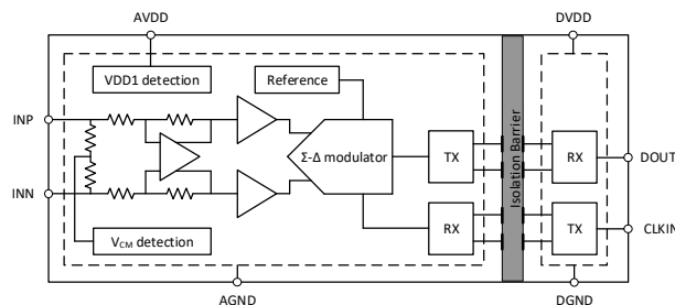
Figure 1. NSI1306C Block Diagram
