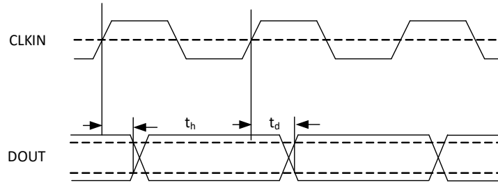
Figure 5.1 Digital Input and Output Timing
