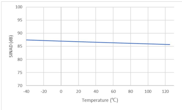
Figure 5.17 Signal-to-Noise + Distortion vs Temperature
