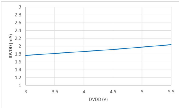
Figure 5.24 Digital Side Supply Current vs Supply Voltage
