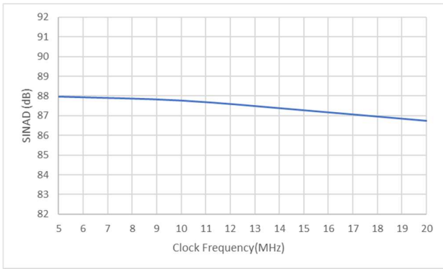
Figure 5.16 Signal-to-Noise + Distortion vs Clock Frequency
