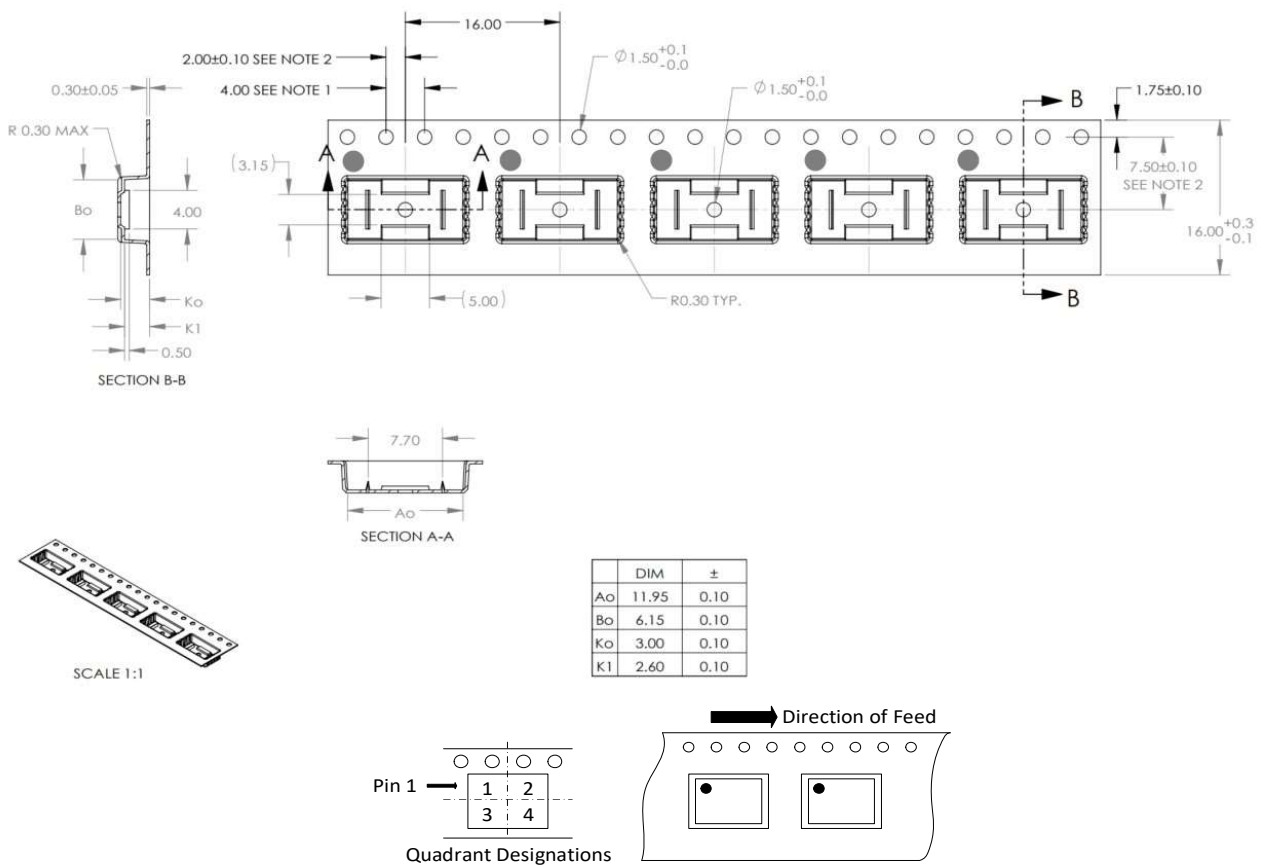
Figure 12.2 Reel Information of SOP8(300mil)
