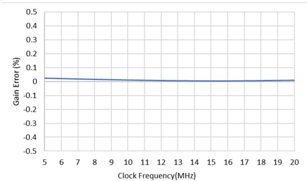
Figure 5.8 Gain Error vs Clock Frequency
