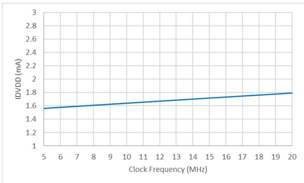
Figure 5.25 Digital Side Supply Current vs Clock Frequency
