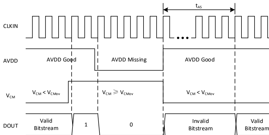
Figure 7.2 Fail-safe output
