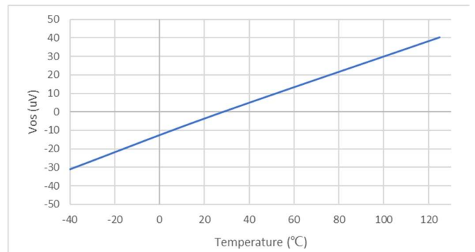
Figure 5.5 Input Offset Voltage vs Temperature
