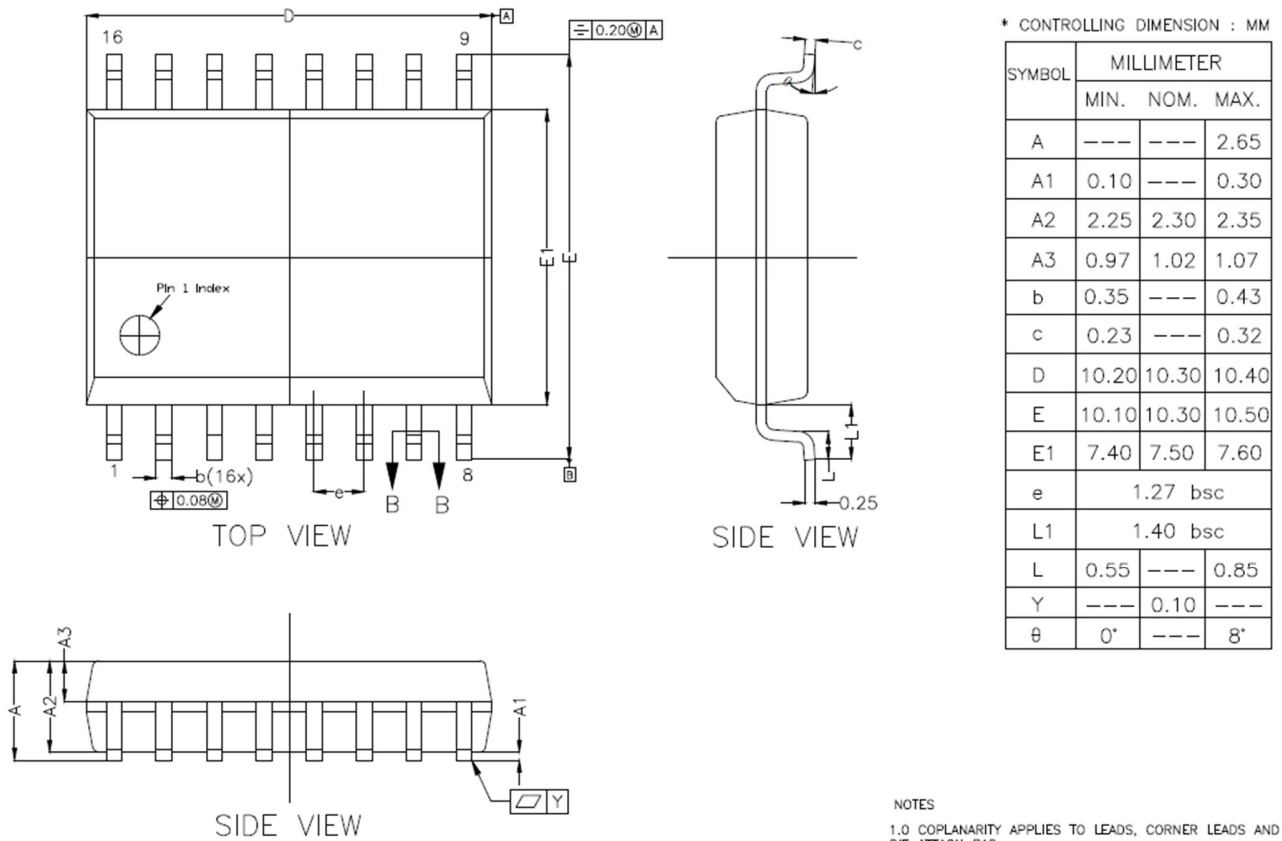
Figure 9.3 SOW16 package shape and dimension in millimeters
