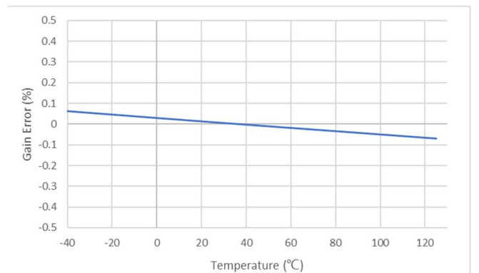
Figure 5.7 Gain Error vs Temperature
