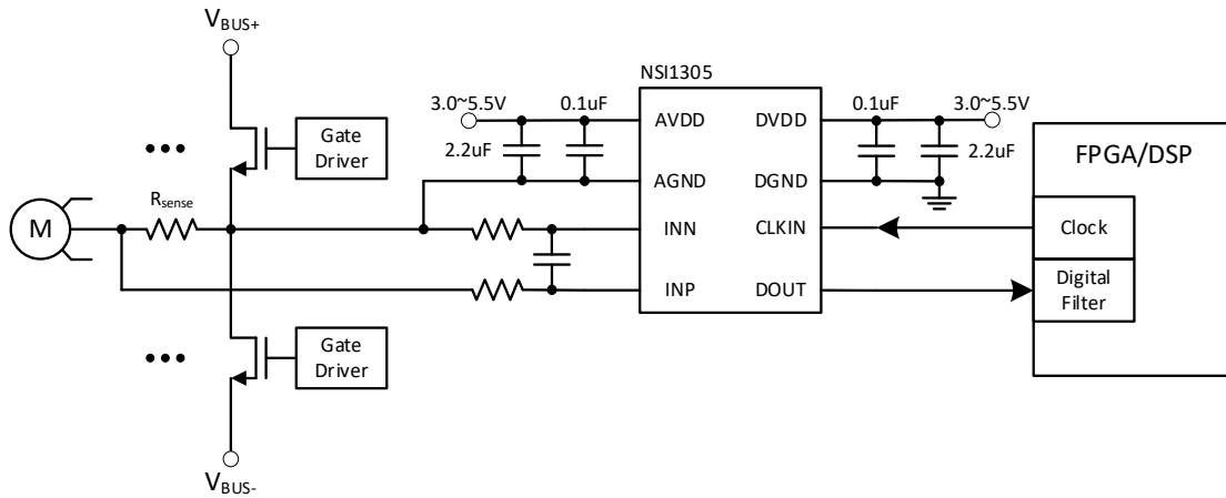
Figure 9.1 Typical application circuit in phase current sensing
