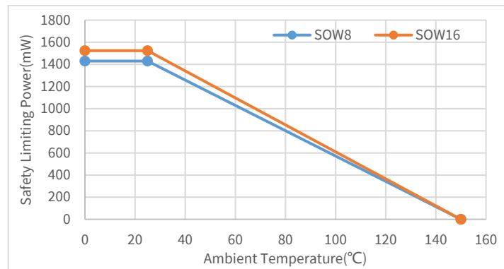
Figure 7.1 NSI1305 Thermal Derating Curve, Dependence of Safety Limiting Values with Case Temperature per DIN VDE V 0884-11
