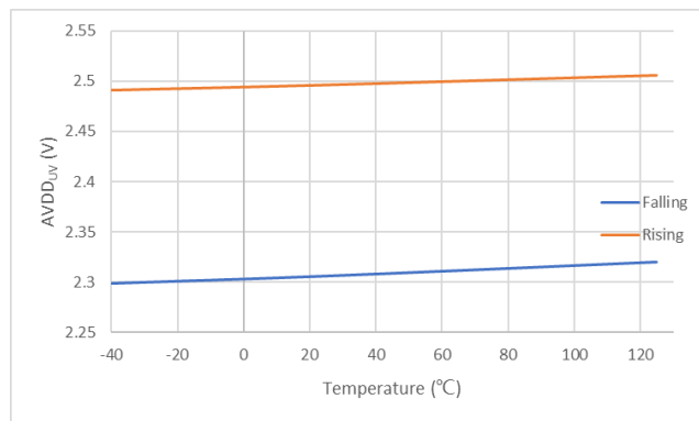
Figure 6.21 Analog Side Under-Voltage Detection Level vs Temperature
