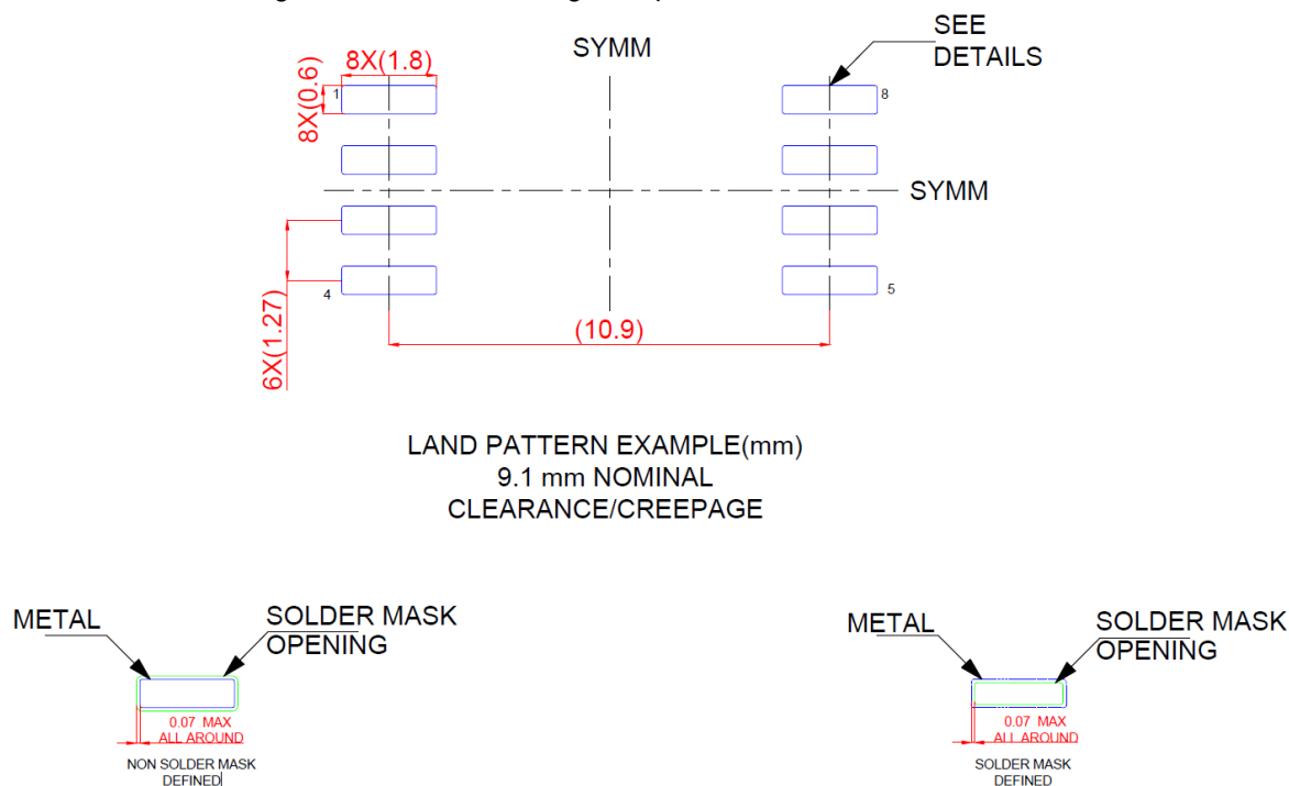
Figure 10.2 SOW8 Package Board Layout Example
