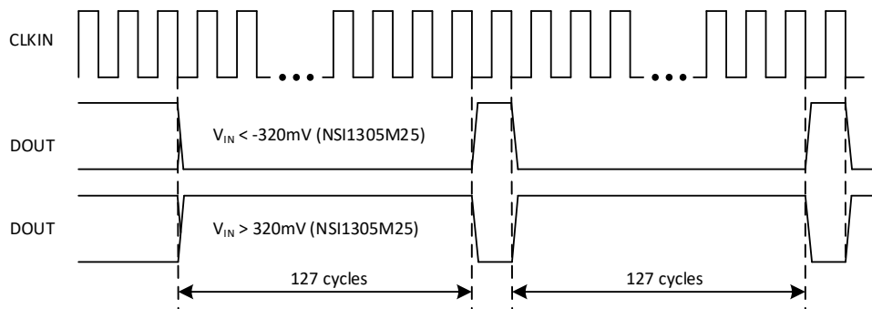
Figure 8.3 Overrange output
