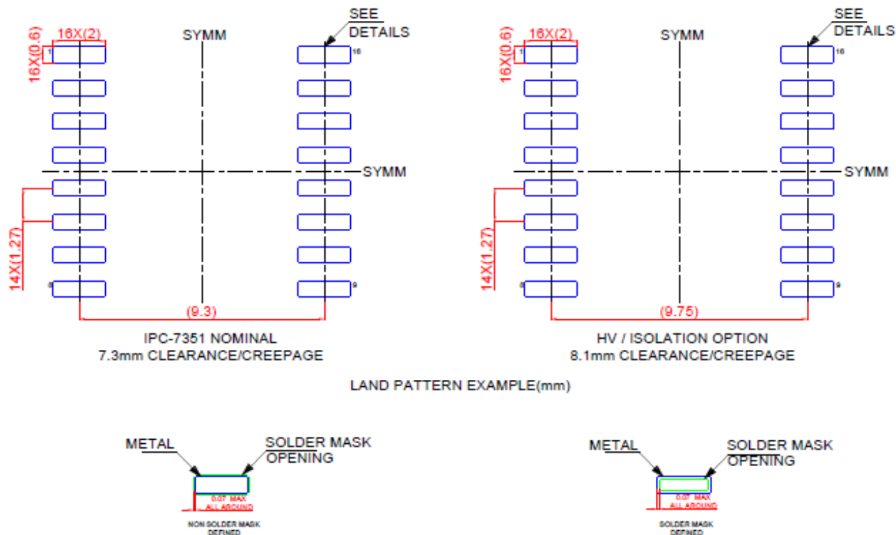
Figure 10.4 SOW16 Package Board Layout Example
