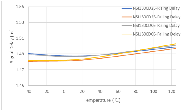
Figure 5.1421 Vin to Vout Delay vs Temperature
