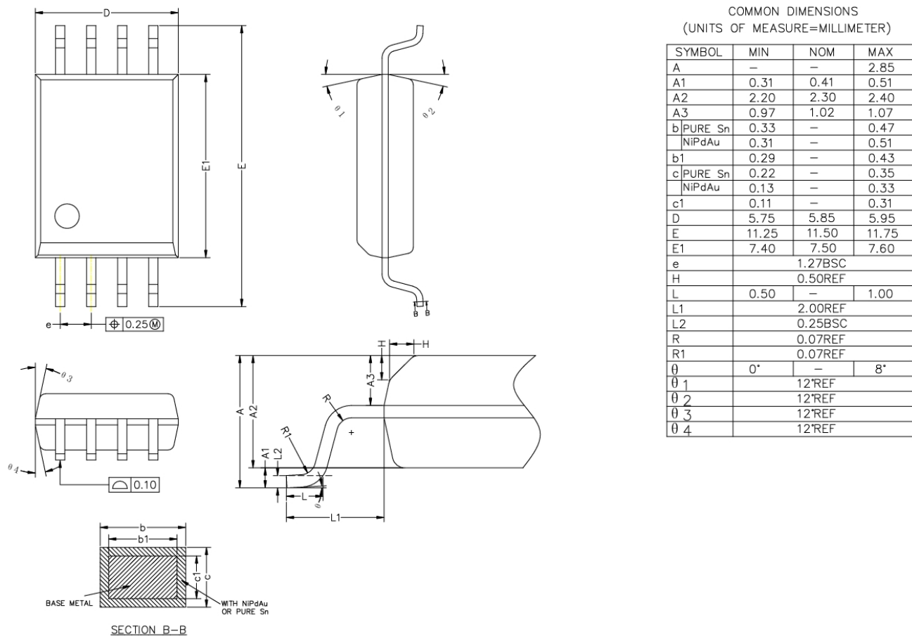
Figure 9.1 SOW8 Package Shape and Dimension in millimeters
