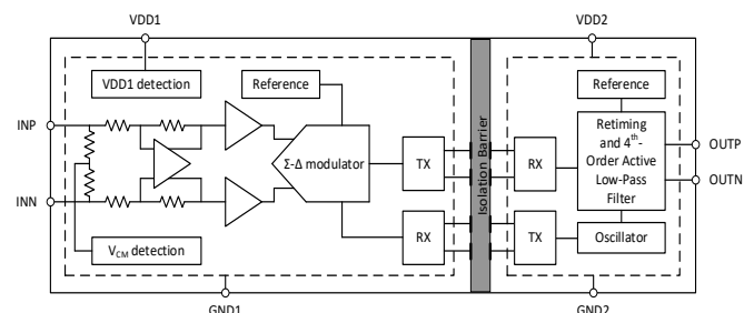
Figure 1. NSI1300 Block Diagram
