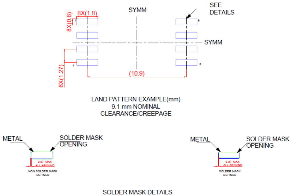
Figure 9.2 SOW8 Package Board Layout Example
