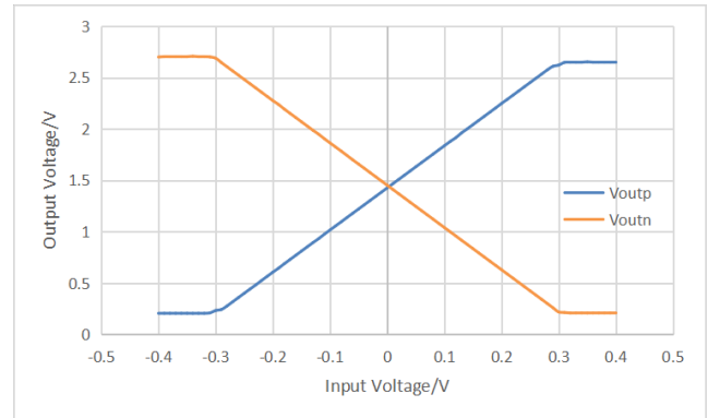
Figure 5.26 Output Voltage vs Input Voltage (NSI1300D25)
