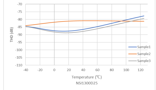
Figure 5.11 THD vs Temperature (NSI1300D25)
