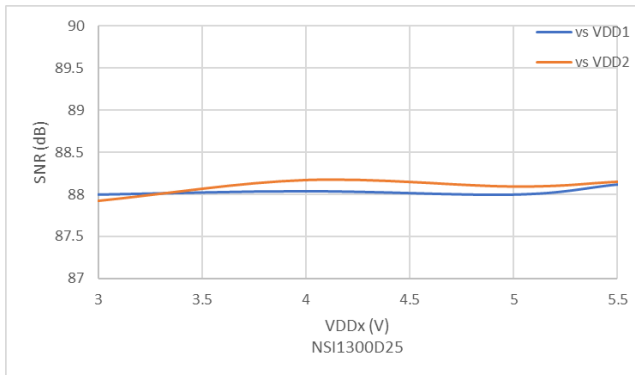
Figure 5.16 SNR vs Supply Voltage (NSI1300D25)
