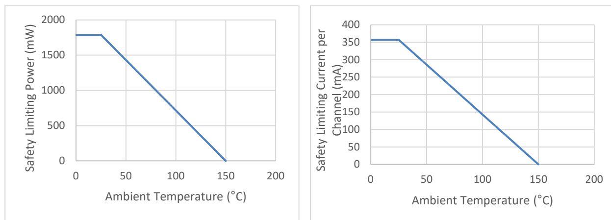
Figure 7.2 NSI1042C-DSWR Thermal derating Curve, Dependence of Safety Limiting Values with Case Temperature per DIN EN IEC 60747-17 (VDE 0884-17)
