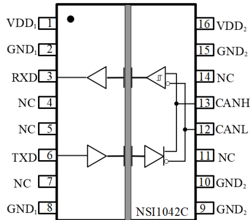
Figure 1.1 NSI1042C-DSWR Package
