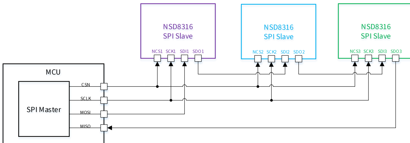
Figure 7.7 Daisy Chain Operation for 3 Devices
