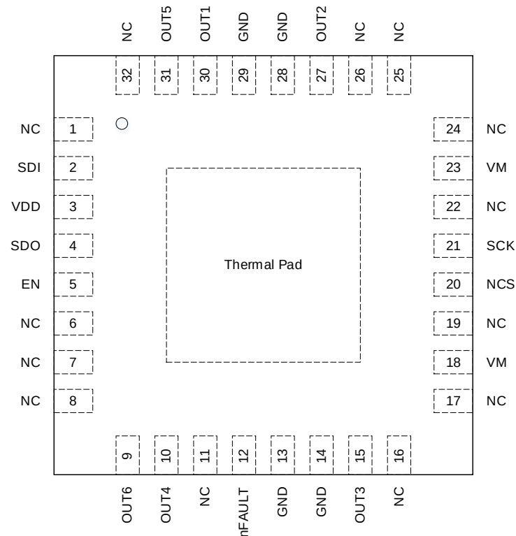
Figure 1.2 NSD8316 VQFN32 Package Pinout
