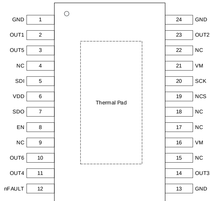
Figure 1.1 NSD8316 HTSSOP24, HTSOP24 Package Pinout
