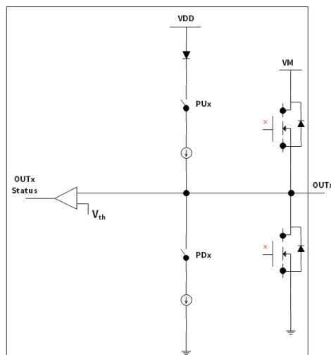
Figure 7.5 Half – Bridge diagnosis OFF-STATE
