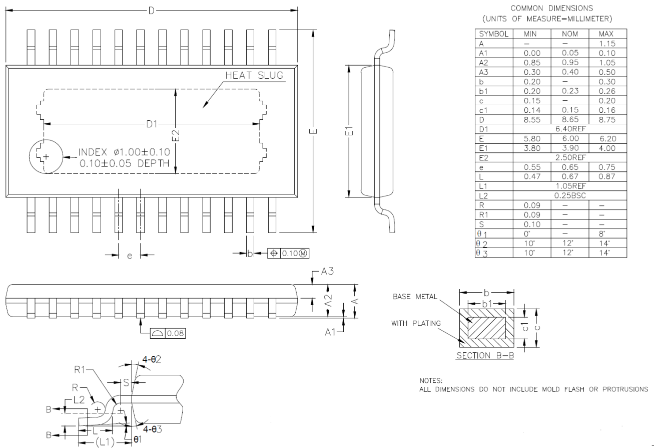
Figure 9.2 HTSOP24 package information
