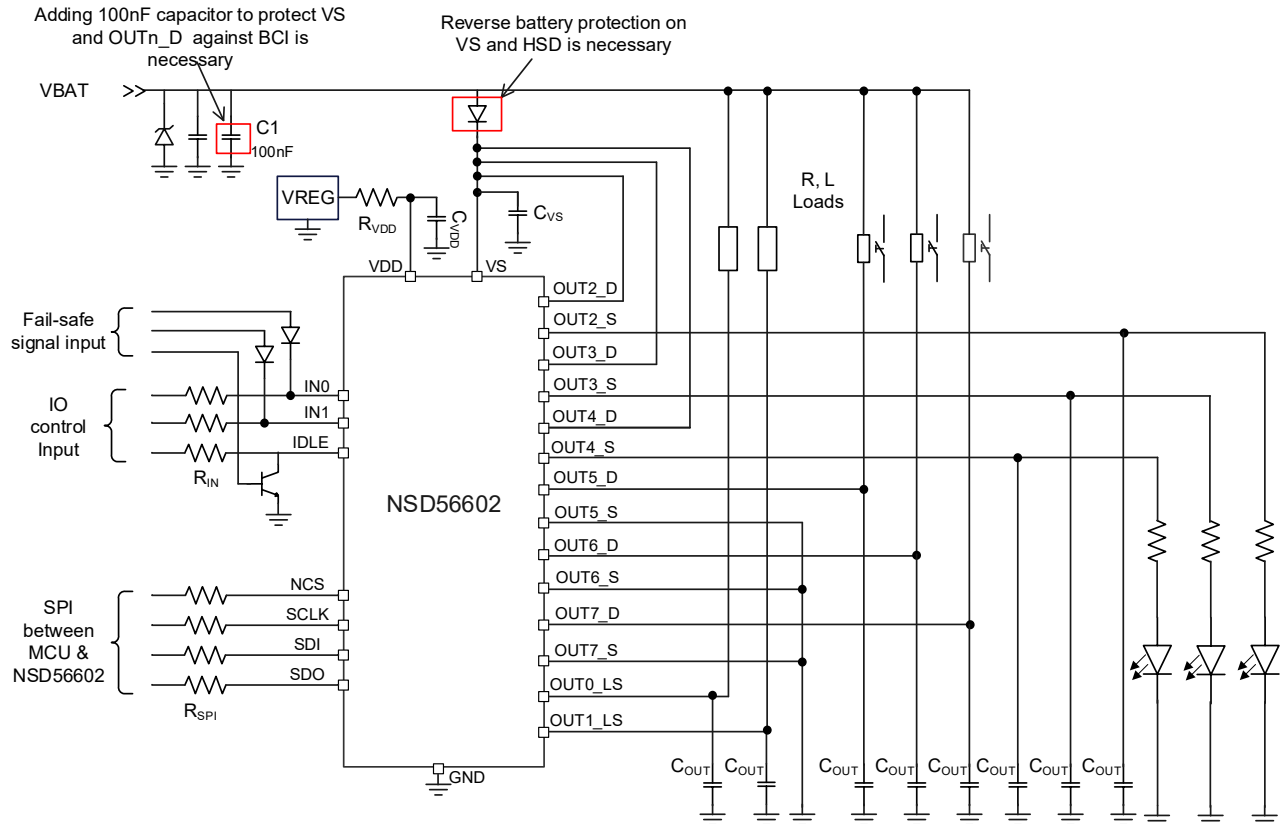
Figure 3.1 NSD56602 Application Diagram
