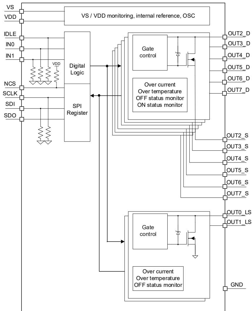
Figure 2.1 Block Diagram of NSD56602
