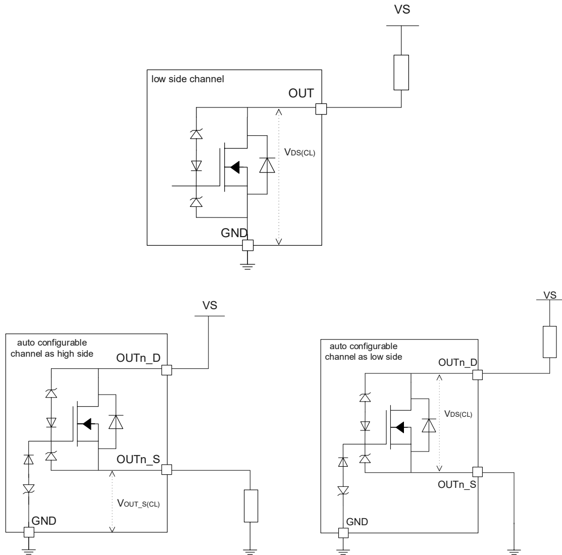
Figure 7.2 Output Clamp concept
