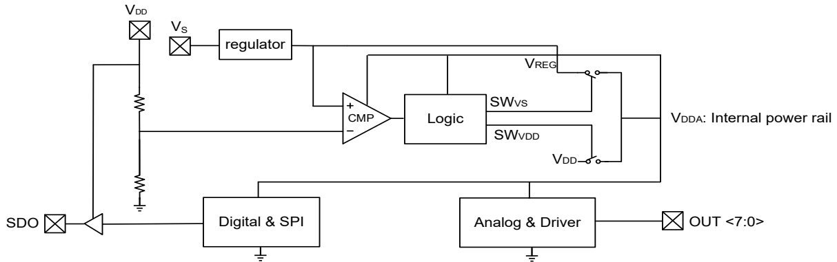
Figure 5.1 NSD56602 Internal Power Supply concept
