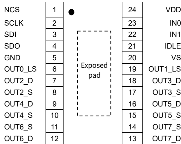
Figure 1.1 Pin Configuration NSD56602 in HTSOP24(Top View)
