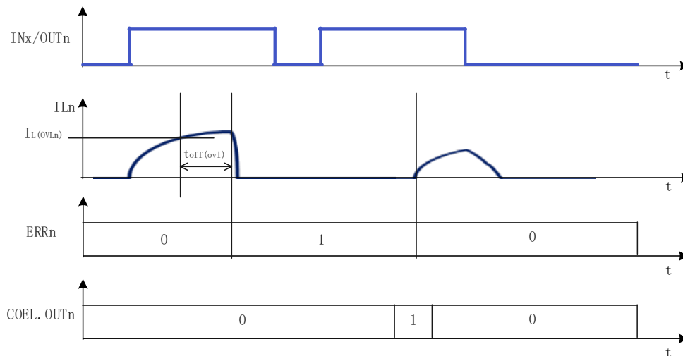
Figure 8.2 Latch OFF at Over Load
