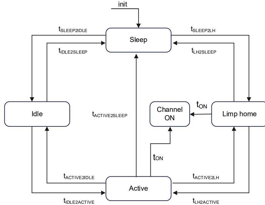
Figure 5.3 Transition Time diagram
