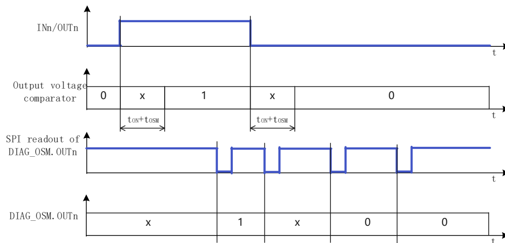
Figure 9.1 Output Status Monitor timing
