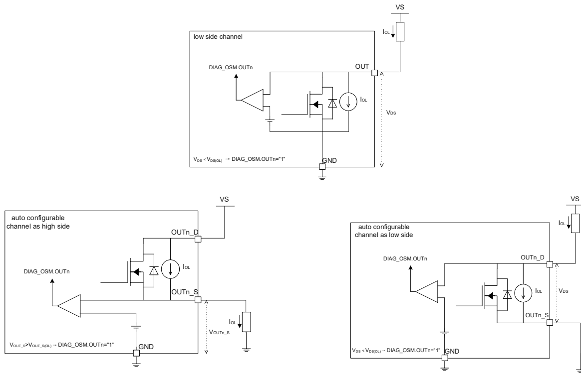
Figure 9.2 Output Status Monitor - concept
