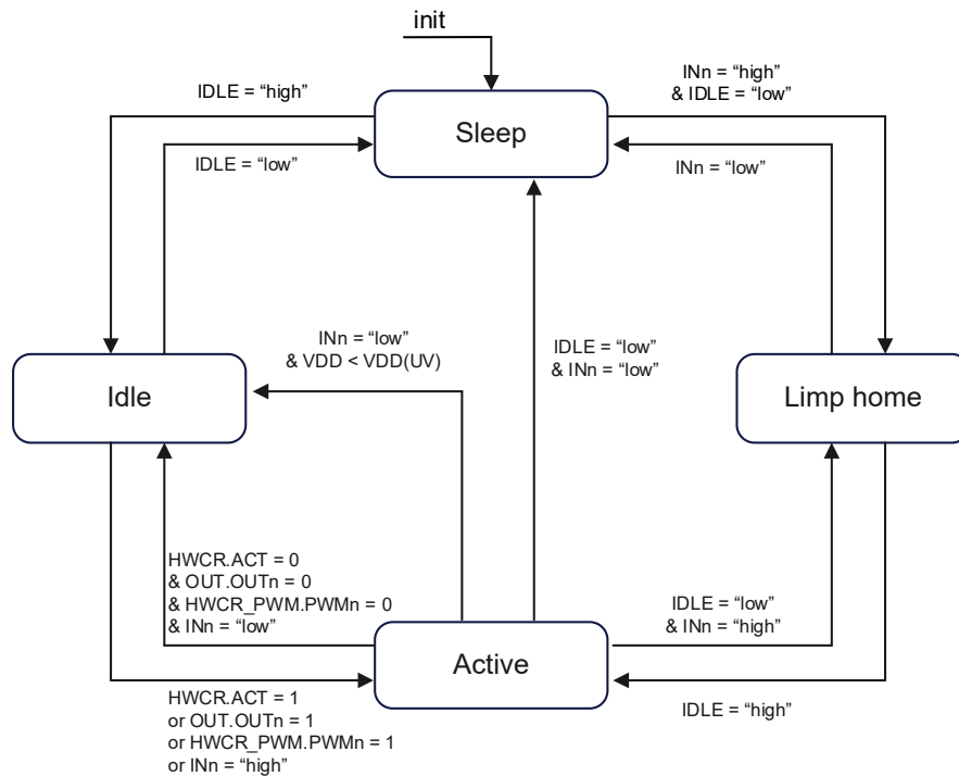
Figure 5.2 Operation Mode state diagram
