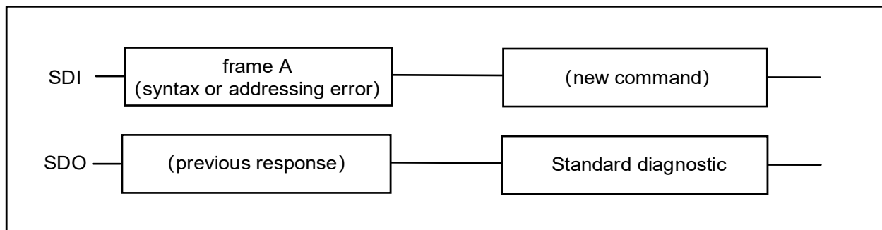
Figure 10.10 NSD56602 response after a command syntax error
