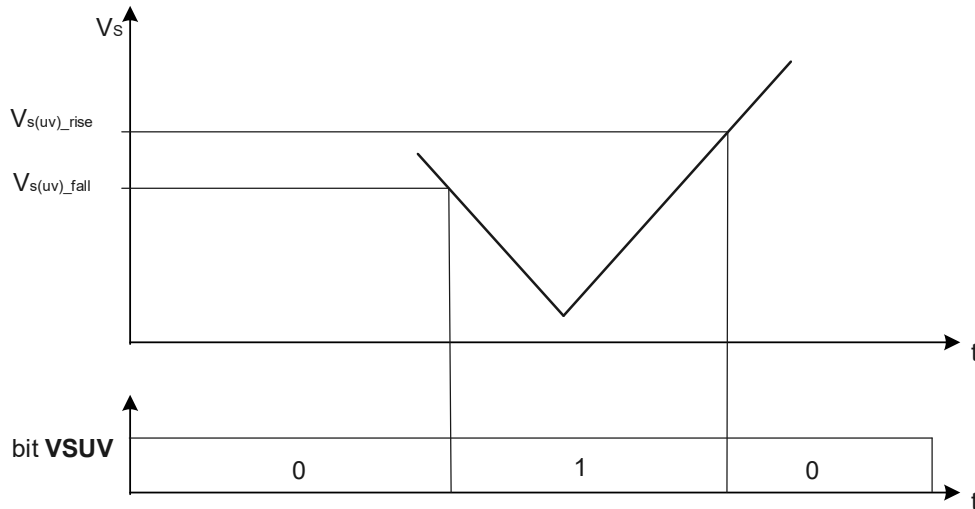
Figure 5.4 VS Undervoltage Behavior
