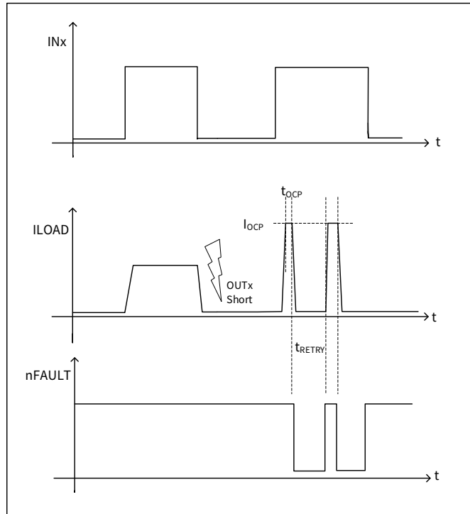
Figure 7.1 Overcurrent Iocp, tOCP & tRETRY behavior
