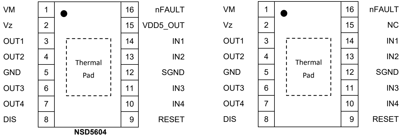
Figure 1.1 NSD5604 and NSD5604N Pinout
