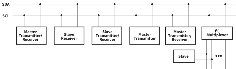
Figure 7.4 System Configuration
