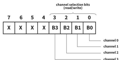
Figure 7.9 Control Register
