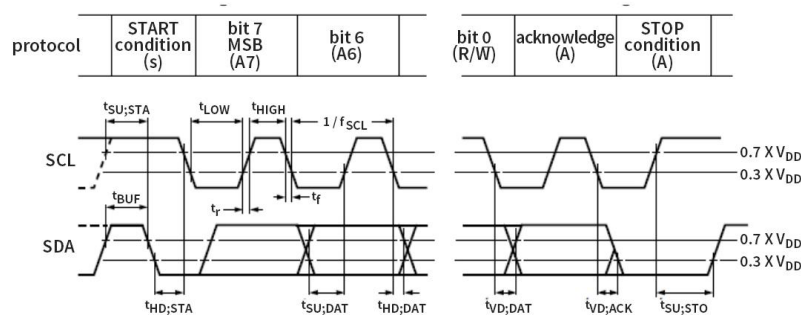
Figure 6.3 I²C-bus timing diagram
