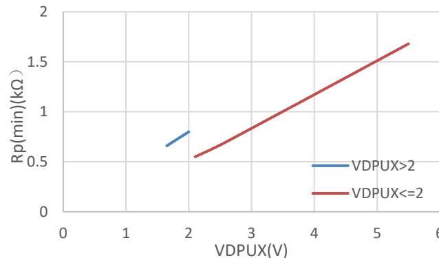
V_{OL}=0.2 \times V_{DPUX} , I_{OL}=2 mA when V_{DPUX} \leq 2 V; V_{OL}=0.4 V, I_{OL}=3 mA when V_{DPUX} > 2 V Figure 8.4 Minimum Pull-Up resistance ( R_{p(min)} ) vs Pull-up reference voltage ( V_{DPUX} )
