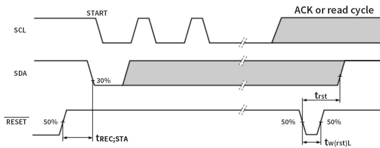
Figure 6.2 Definition of RESET timing
