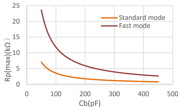
Standard mode ( f_{SCL}=100 kHz, t_r=1 μs); Fast mode: ( f_{SCL}=400 kHz, t_r=300 ns) Figure 8.3 Maximum Pull-Up resistance ( R_{p(max)} ) vs Bus Capacitance ( C_b )
