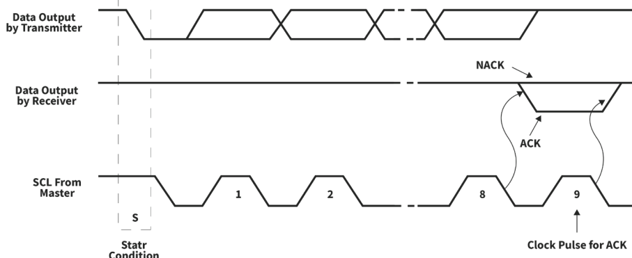
Figure 7.5 Acknowledgment on the I²C Bus
