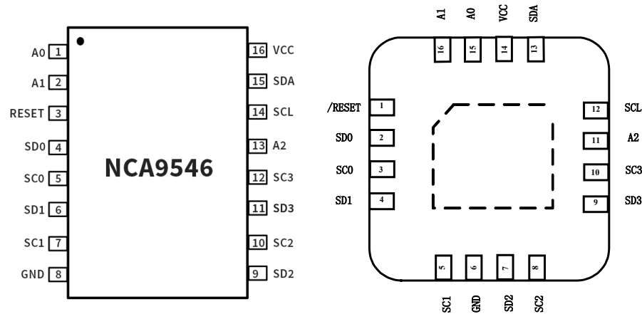
Figure 1.1 NCA9546 Package
