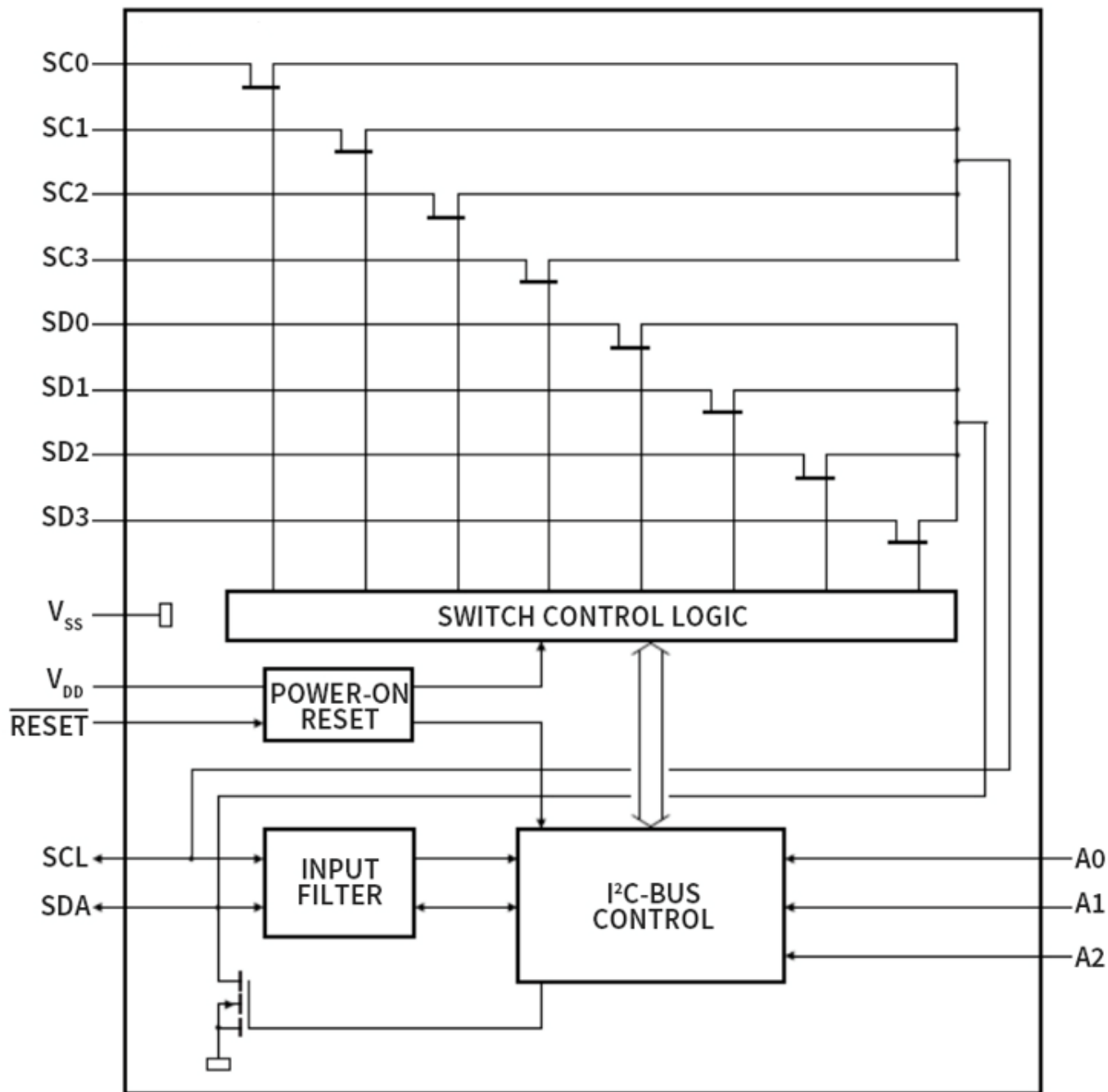
Figure 7.1 NCA9546 Functional block
