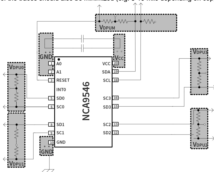
Figure 9.1 Typical Application PCB
