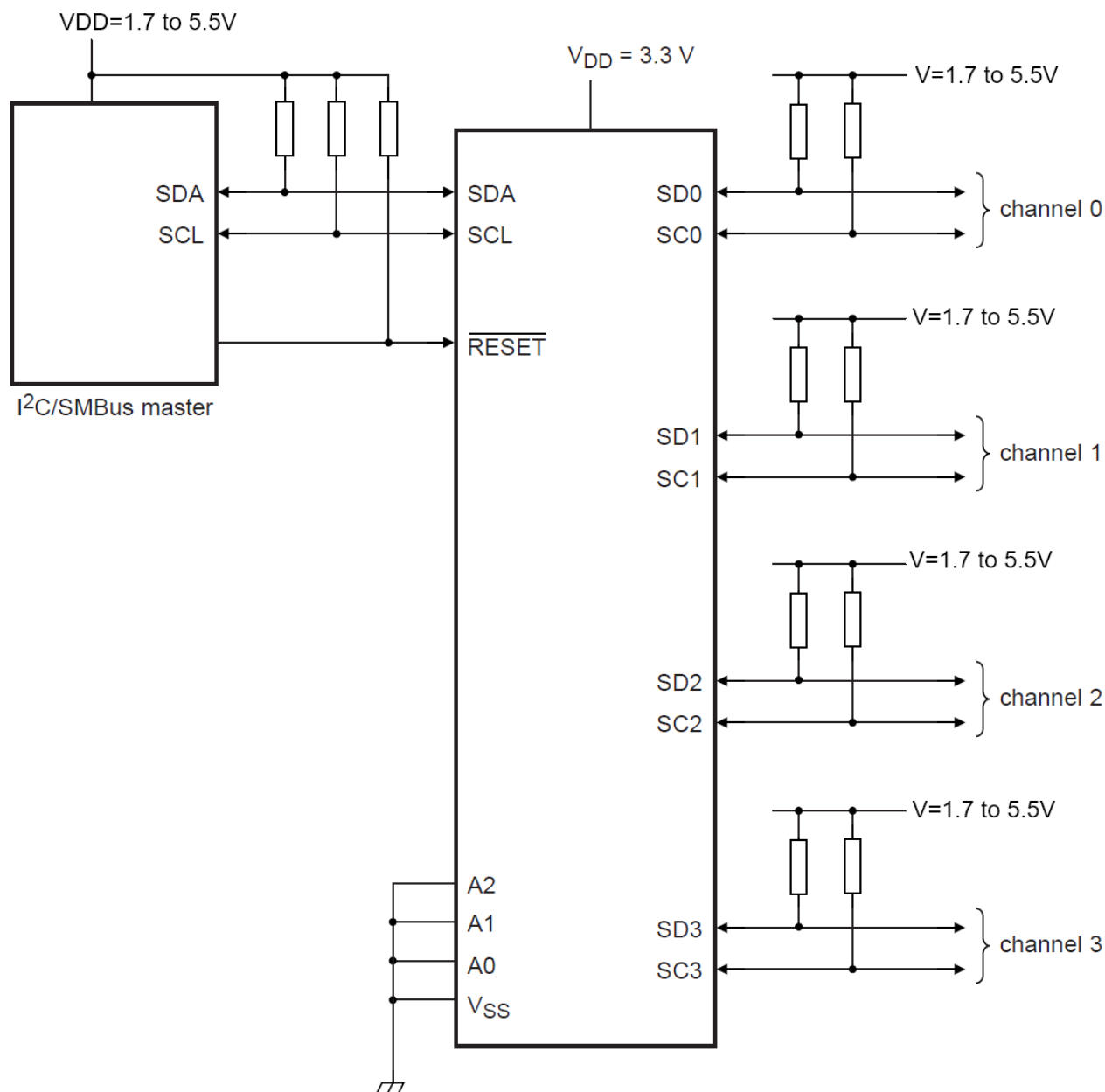
Figure 8.1 Typical Application Schematic
