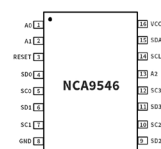
Figure 1. NCA9546 pin configuration
