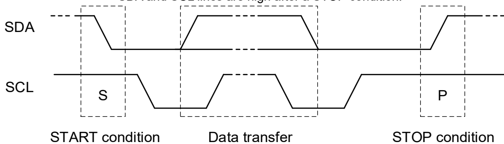
Figure 7-4. Definition of START and STOP conditions
