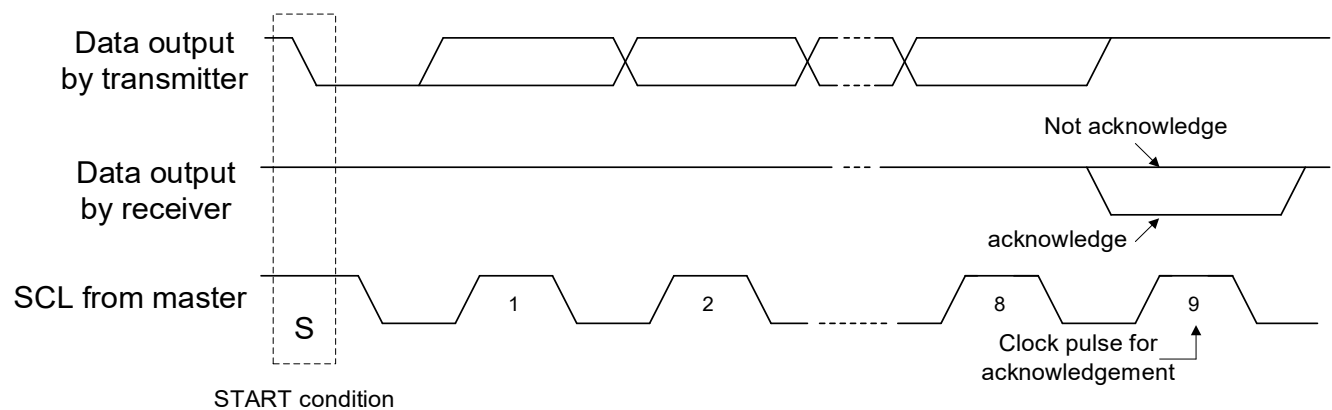
Figure 7-7. Acknowledgement on I 2 C-bus
