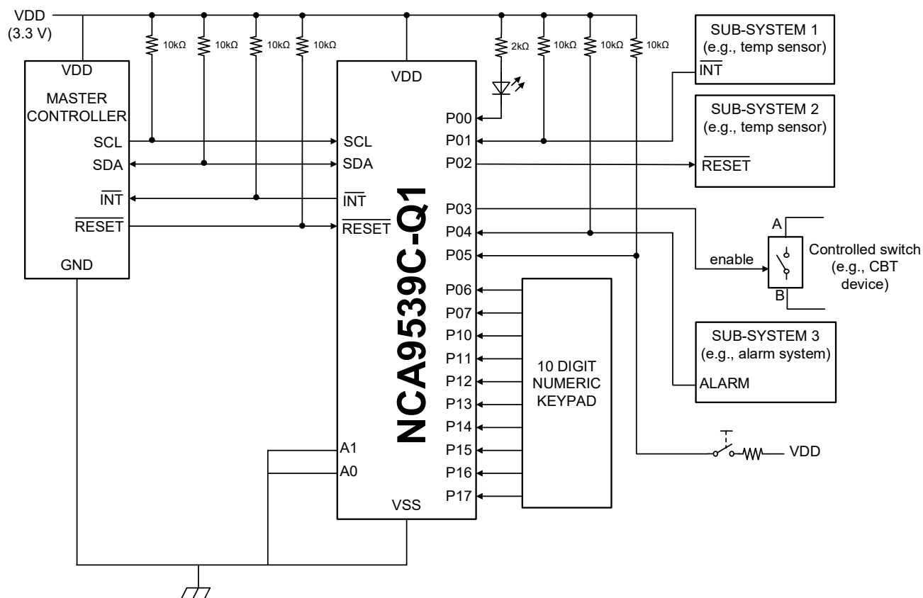
Figure 8-1. Typical Application
