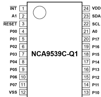
Figure 1. NCA9539C-Q1TSXR Pinout
