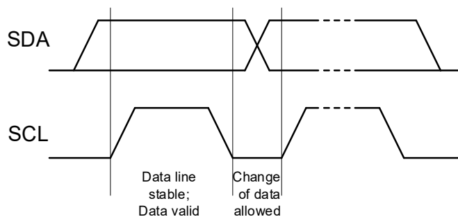
Figure 7-5. Bit transfer
