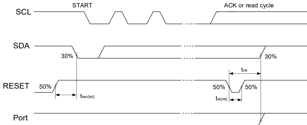
Figure 7-3. Definition of RESET\ timing
