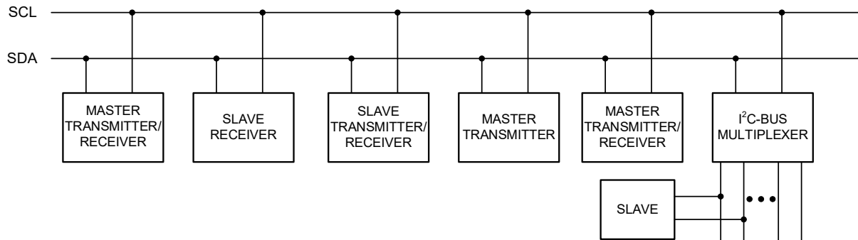
Figure 7-6. System configuration
