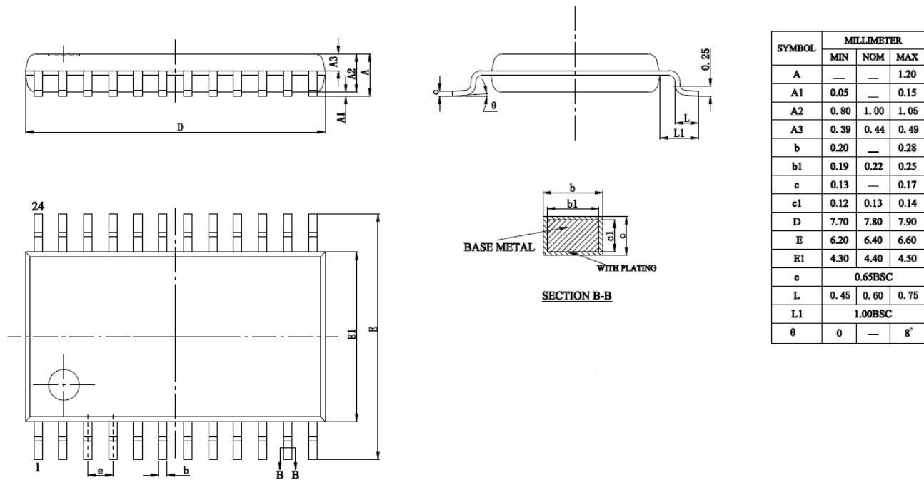
Figure 11-2. TSSOP24 Package Shape and Dimension in millimeters
