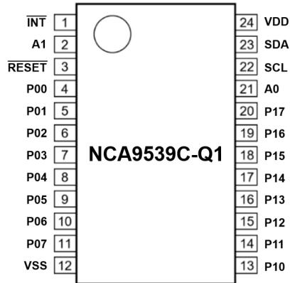
Figure 1-1. NCA9539C-Q1 Package
