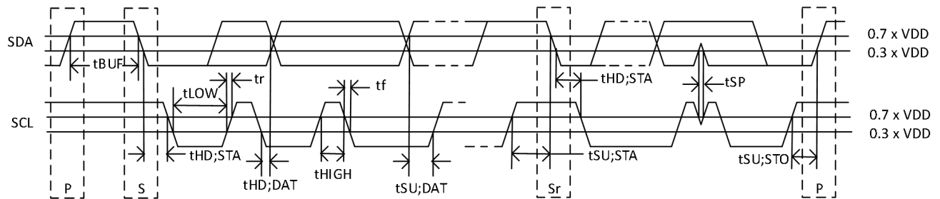
Figure 5. 1 Definition of timing on I²C-bus
