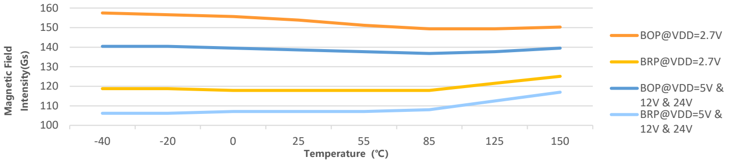
Figure.7 Magnetic Characteristics vs. Temperature & V_{DD} ( B_{OP} & B_{RP} )
