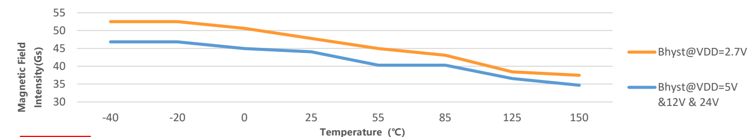
Figure.11 Magnetic Characteristics vs. Temperature & V_{DD} ( B_{HYST} )
