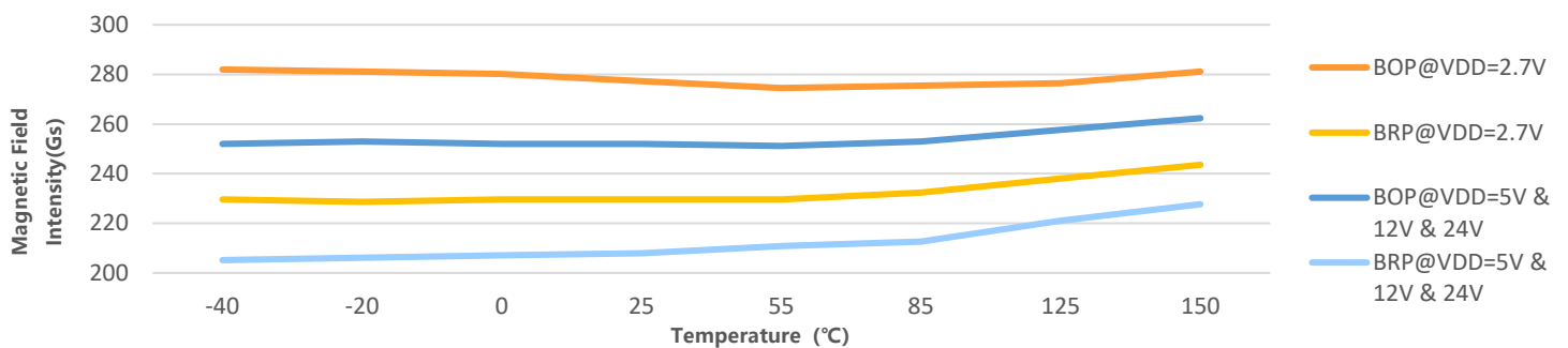
Figure.10 Magnetic Characteristics vs. Temperature & V_{DD} ( B_{OP} & B_{RP} )
