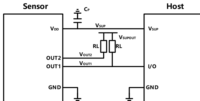
Figure.13 Sensor-Host connection diagram for self-diagnosis function (MT8911AT-Dual as example)
