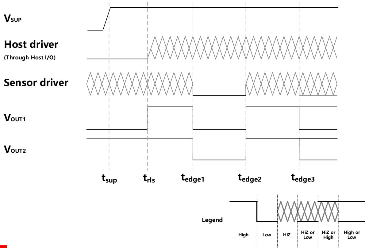
Figure.14 Self-diagnosis timing diagram (MT8911AT-Dual as example)
