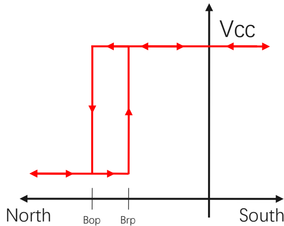
Figure.2 Switching Function Uni-polar (North) SOT-23 & SOT-23-6L
