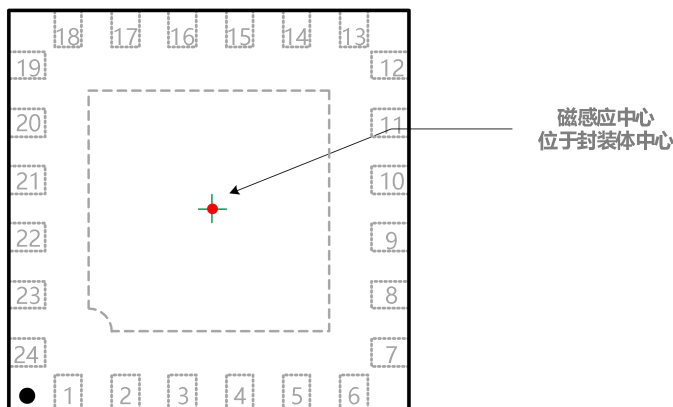
图-2: MT6826S QFN4x4-24L 封装外观图
