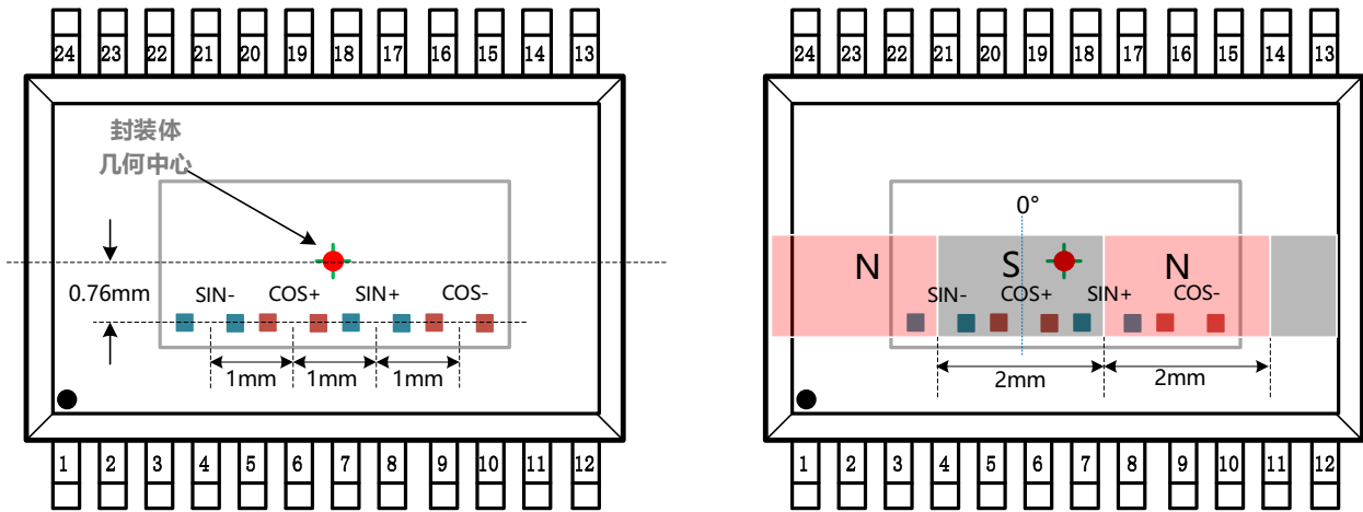
图-1: MT6620GA TSSOP-24封装外观图
