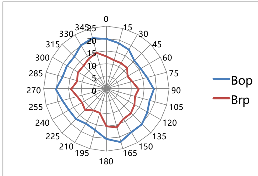
Figure.9 360 Degree Magnetic Characteristics (At V_{CC}=3.6V , T_A=25^\circ C )
