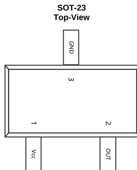
Figure.1 Pin Configuration & Functions
