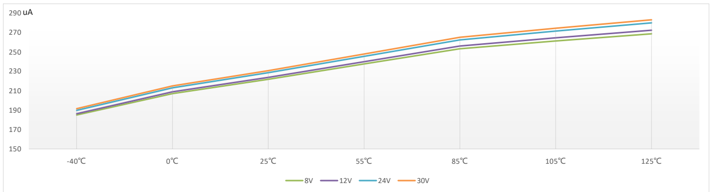
Figure.6 Supply Current vs . Temperature & Vcc
