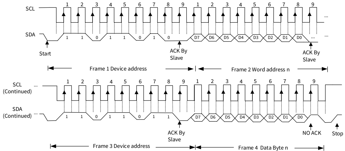
Figure 6.6 I 2 C Read Byte
