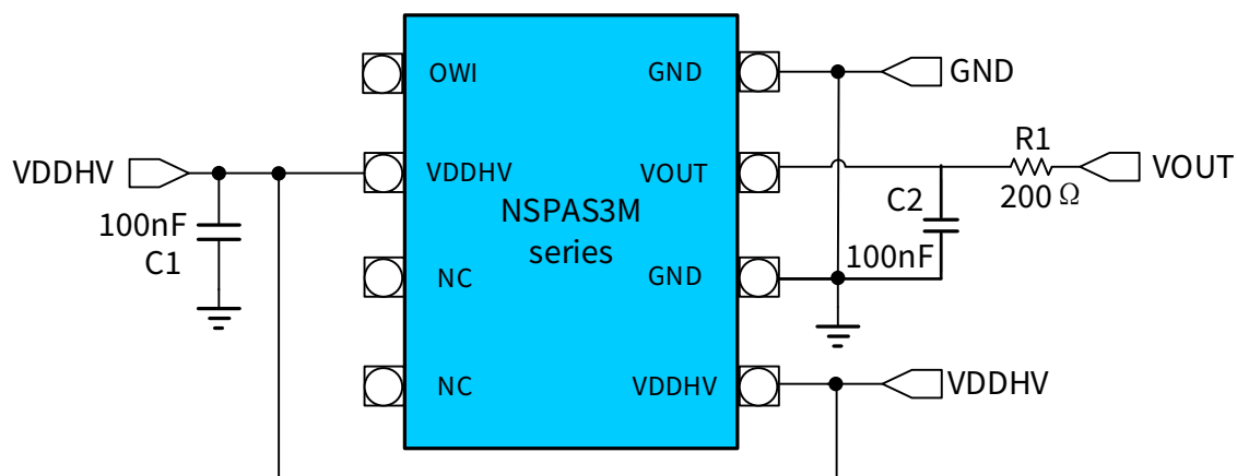
Fig 6.1 Application Circuit
