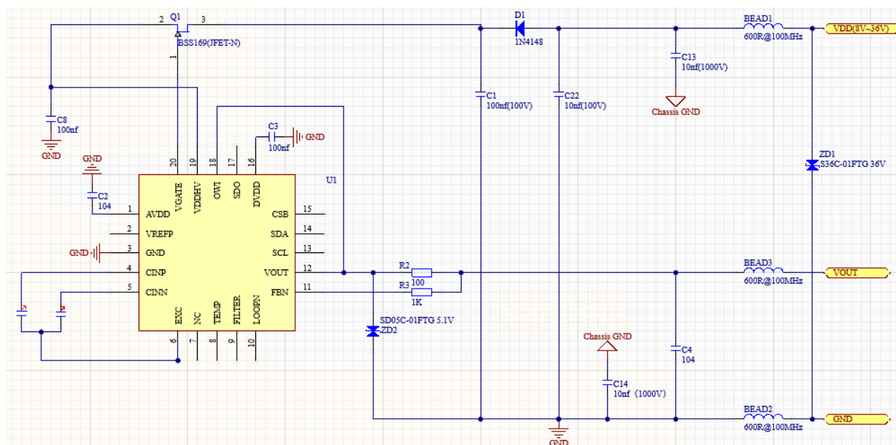
Figure 2. 18 0-5V Typical Application-2
