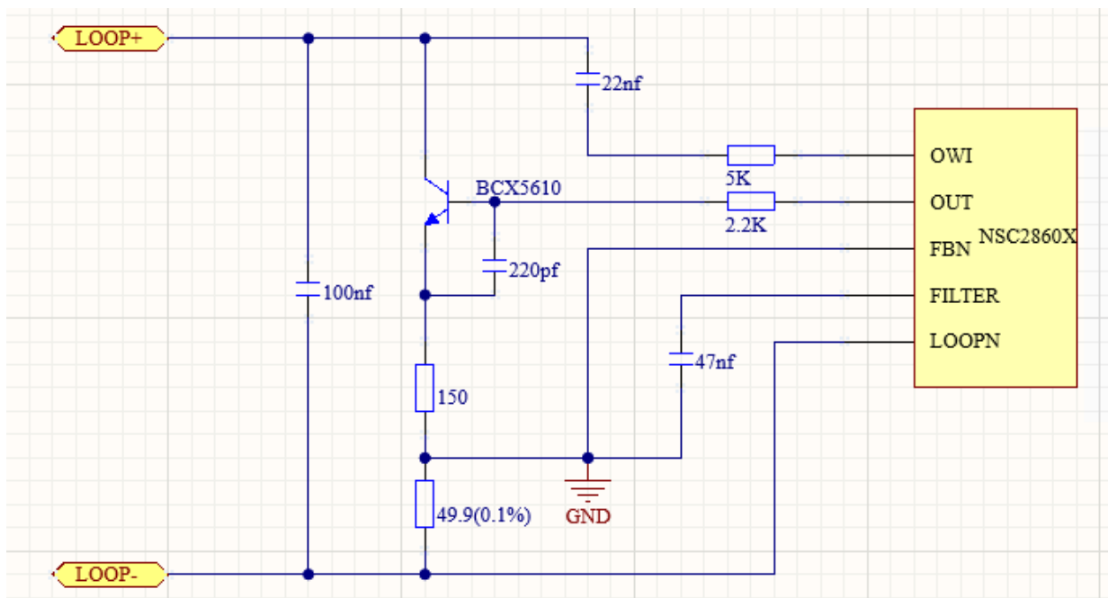
Figure 2. 7 4-20mA Current Output
