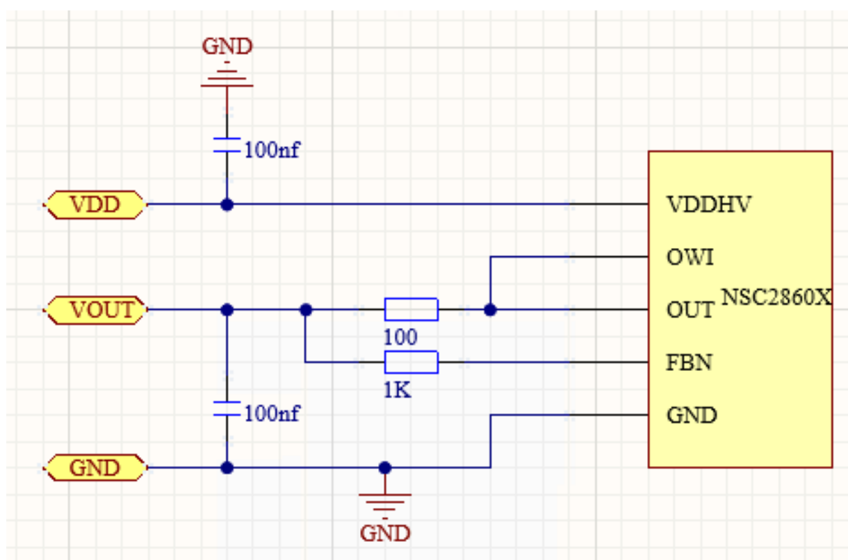
Figure 2. 10 0-5V Voltage Output
