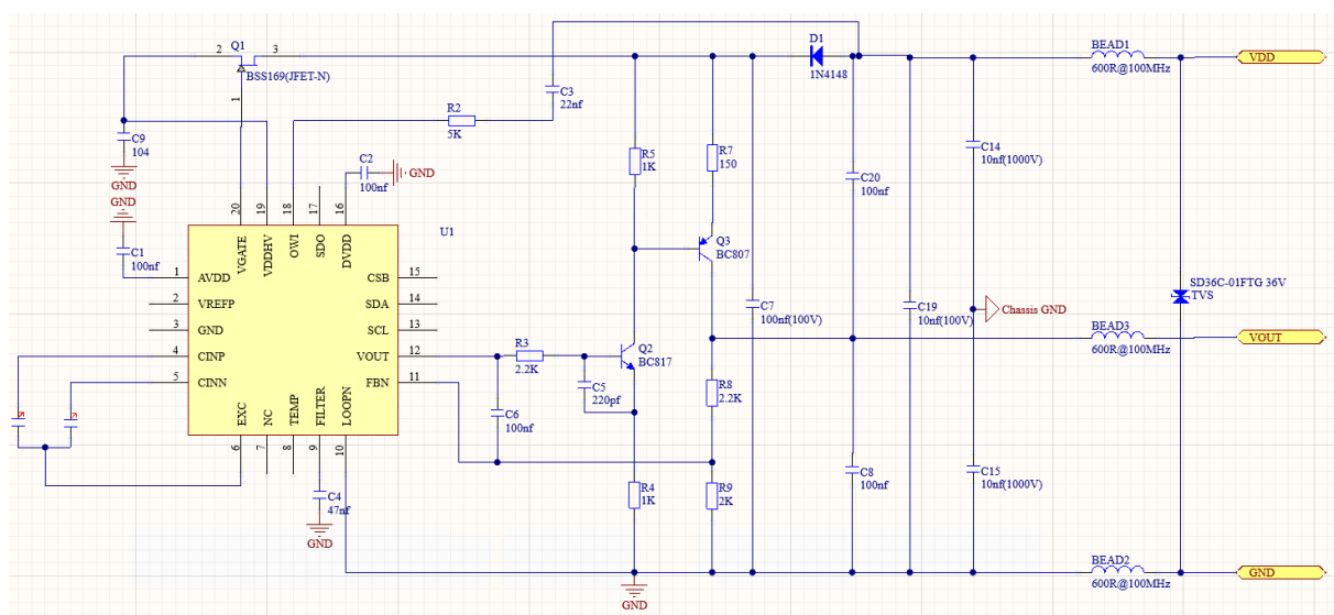
Figure 3.3 0-10V Typical Application-1
