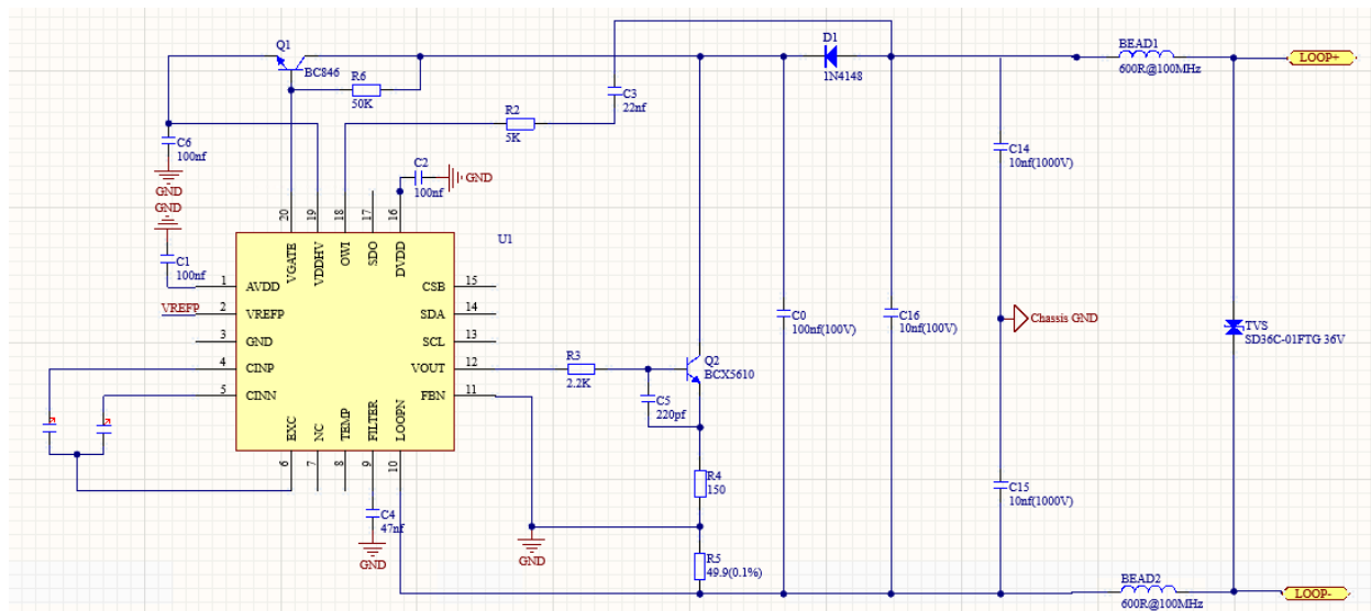
Figure 3.2 4-20mA Typical Application-2
