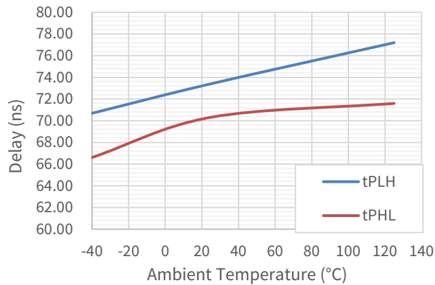
Figure 6.9 Propagation delay versus Temperature
