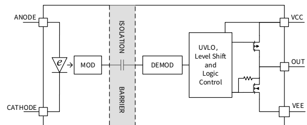
Figure 1. NSI6801E Block Diagram
