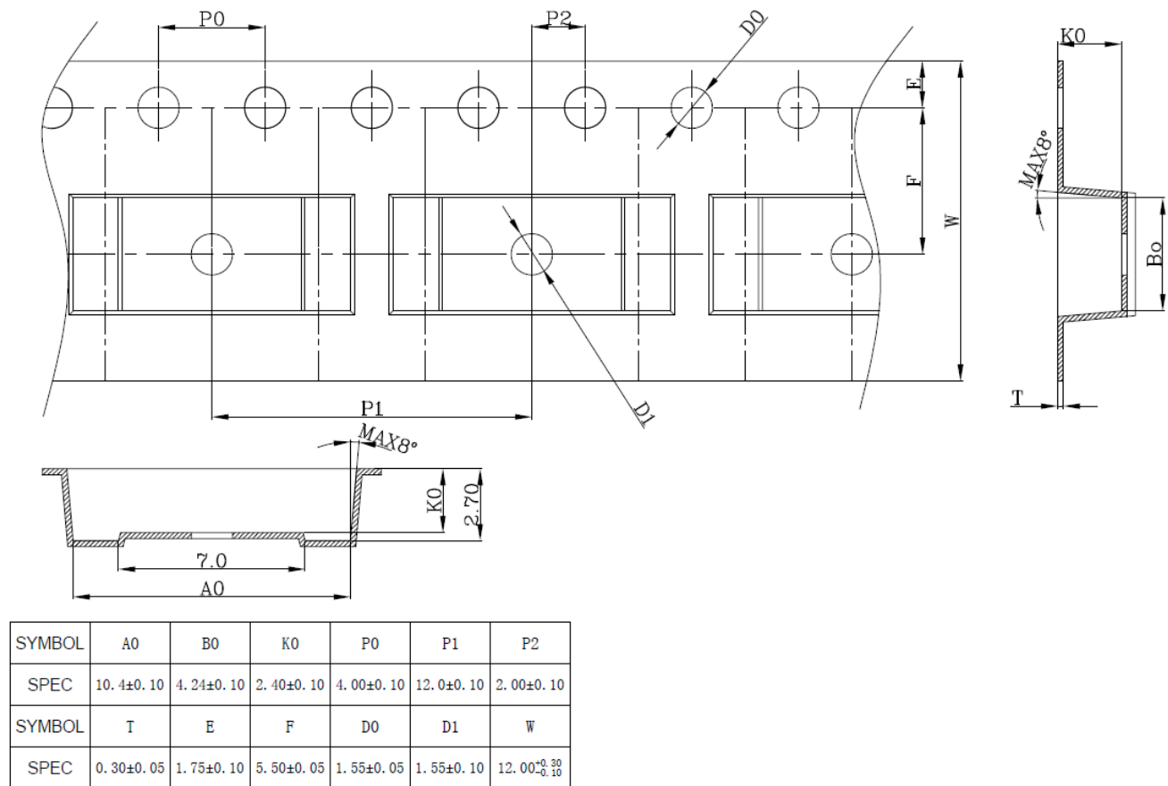
Figure 13.4 Tape Information of SOL6
