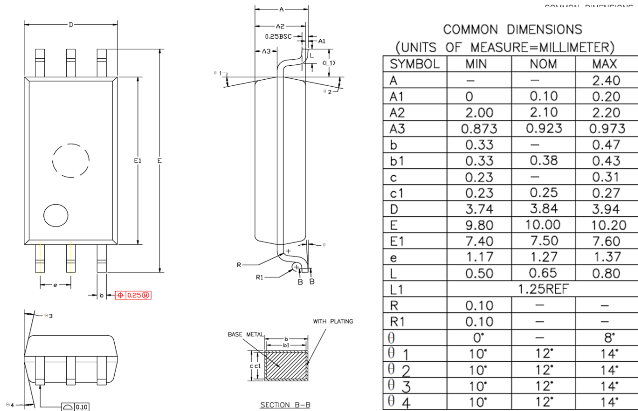
Figure 10.3 SOL6 Package Shape and Dimension in millimeters
