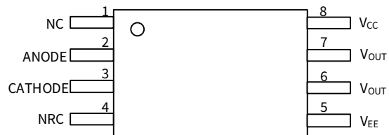
NSI6801ET DUB8 Top View
