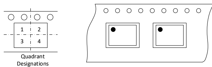
Figure 13.6 Quadrant Designation for Pin1 Orientation in Tape
