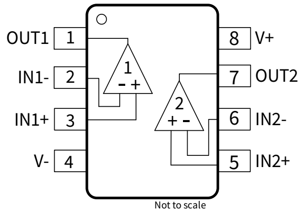
Figure 1-3 NSOPA9102 8-Pin SOP and MSOP Package Top View
