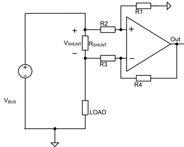
Figure 9-3 High-Side Current Sensing
