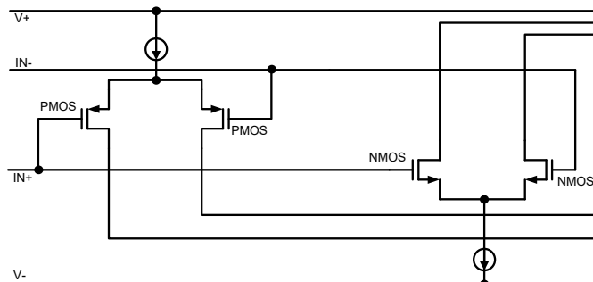
Figure 8-6 NSOPA910x Rail-to-rail Input Stage
