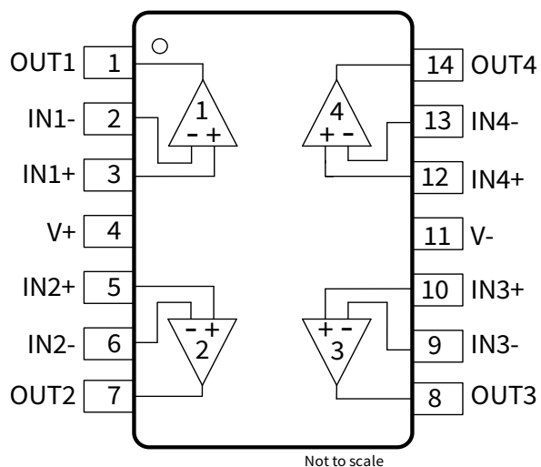
Figure 1-4 NSOPA9104 14-Pin SOP and TSSOP Package Top View
