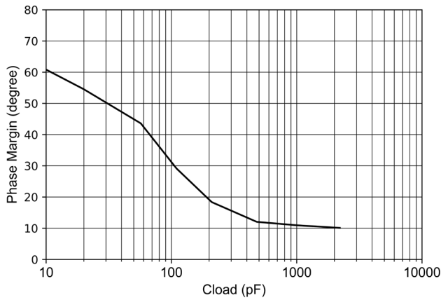
Figure 7-31 Phase Margin vs Capacitance
