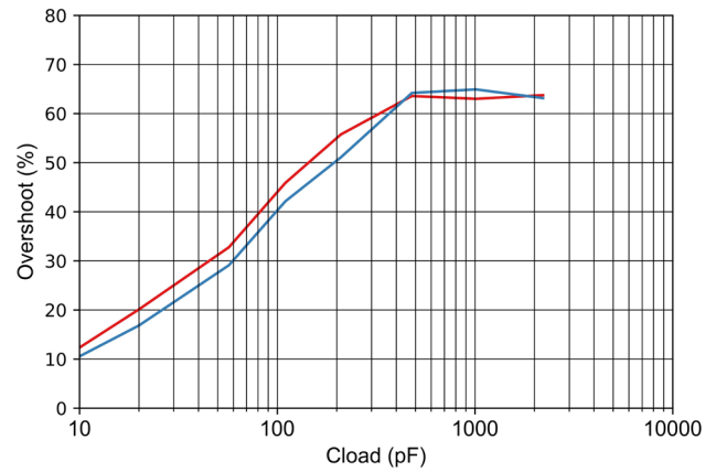
Figure 7-32 Overshoot vs Capacitance
