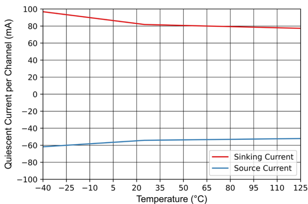
Figure 7-35 Short-Circuit vs Temperature
