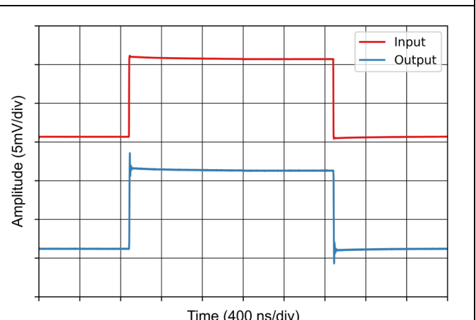
Figure 7-24 Small-Signal Step Response
