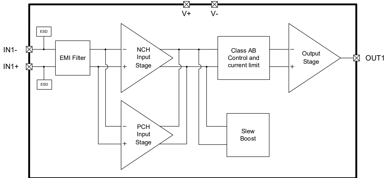
Figure 8-1 NSOPA910x Functional block Diagram (One channel is shown)
