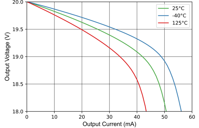
Figure 7-34 Output Voltage Swing vs Output Sourcing Current
