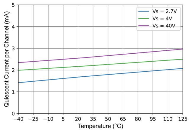
Figure 7-14 Quiescent Current vs Temperature
