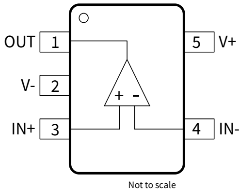
Figure 1-1 NSOPA9101 5-Pin SOT-23 Package Top View
