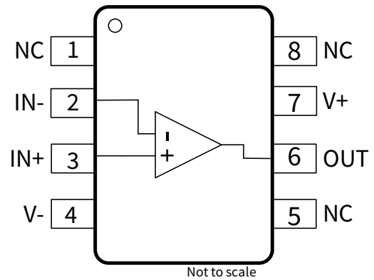
Figure 1-2 NSOPA9101 8-Pin SOP Package Top View
