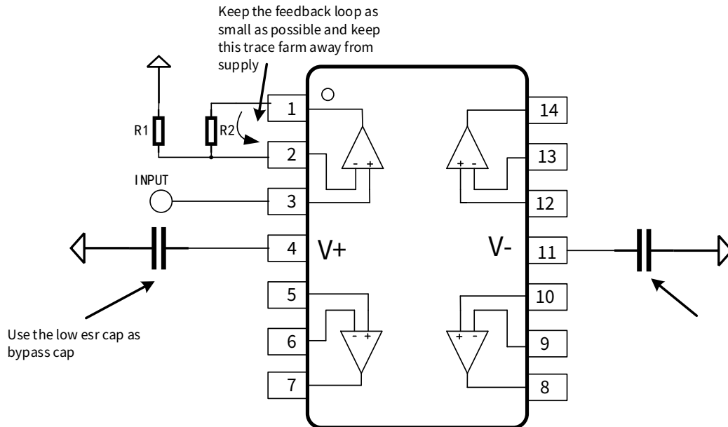
Figure 10-1 Layout example
