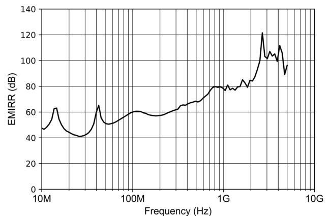
Figure 7-36 EMIRR vs Frequency
