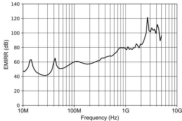
Figure 8-7 NSOPA910x EMIRR vs Frequency
