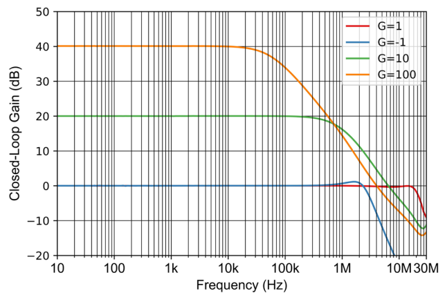
Figure 7-18 Closed Loop Gain and Phase vs Frequency
