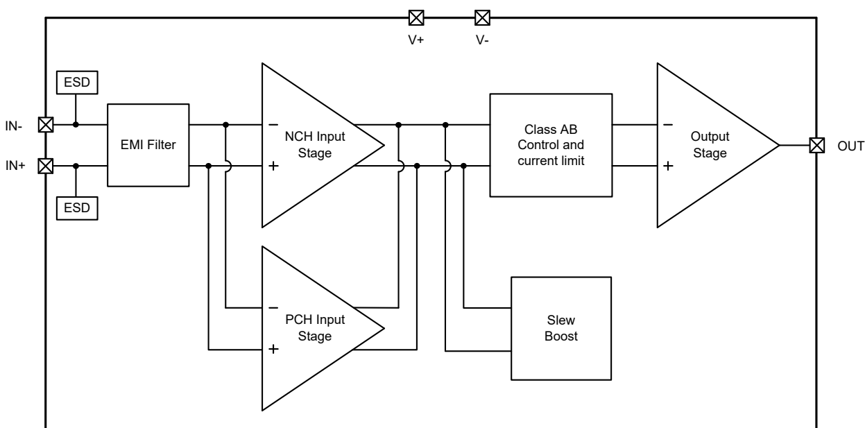
Figure 8-1 NSOPA805x Functional block Diagram (One channel is shown)
