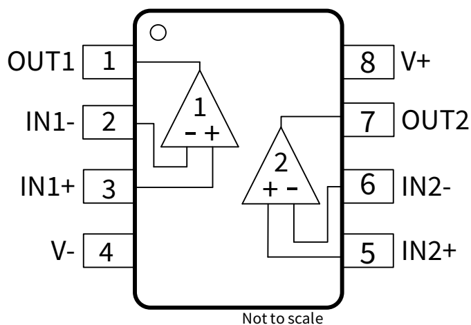
Figure 1-3 NSOPA8052 8-Pin SOP and MSOP Package Top View
