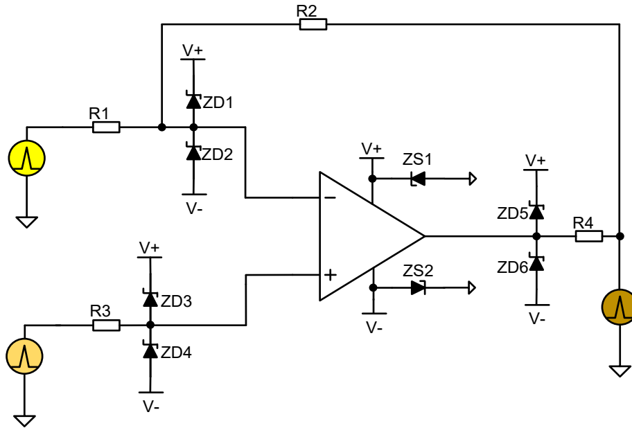
Figure 8-6 External component to enhance EOS performance
