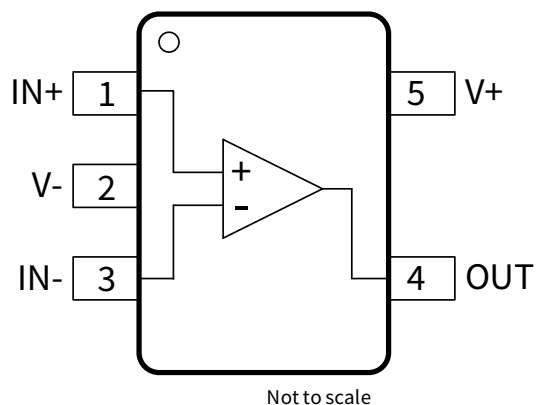
Figure 1-2 NSOPA8051 5-Pin SC70 Package Top View
