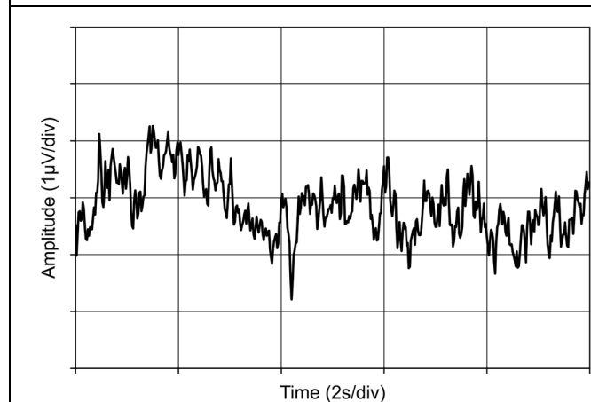
Figure 7-27 0.1-Hz to 10-Hz Noise
