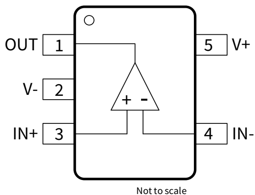
Figure 1-1 NSOPA8051 5-Pin SOT23 Package Top View
