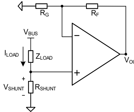
Figure 9-3 NSOPA805x in a Low-Side, Current-Sensing Application
