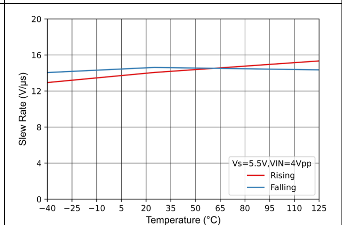
Figure 7-22 Slew Rate vs Temperature
