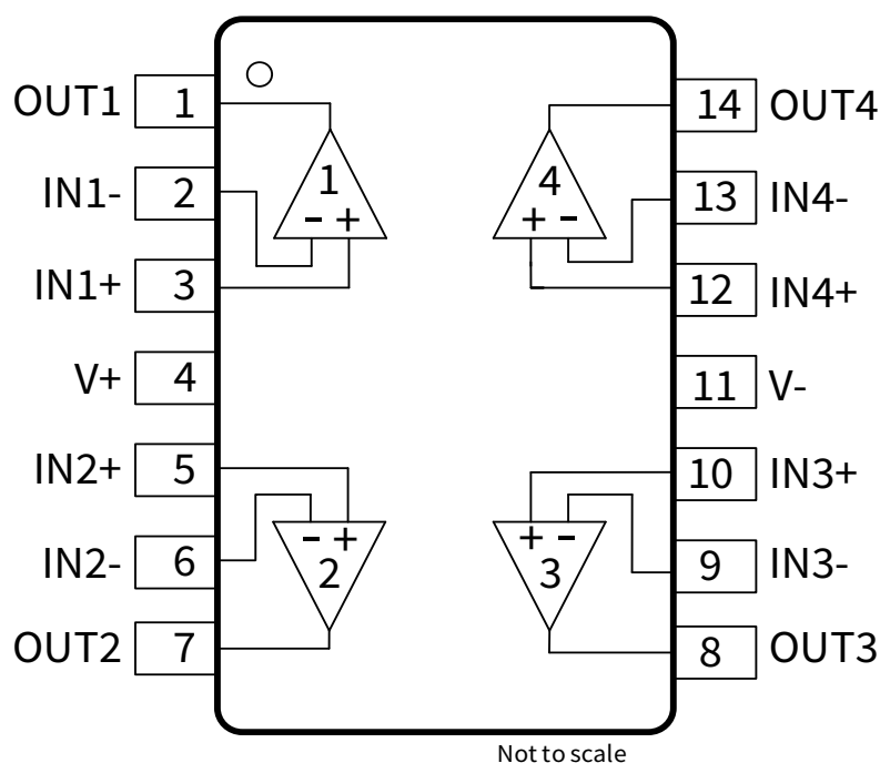
Figure 1-4 NSOPA8054 14-Pin SOP and TSSOP Package Top View
