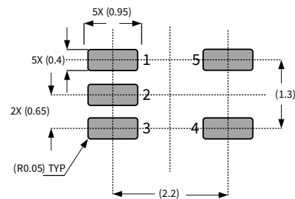
SC70-5
