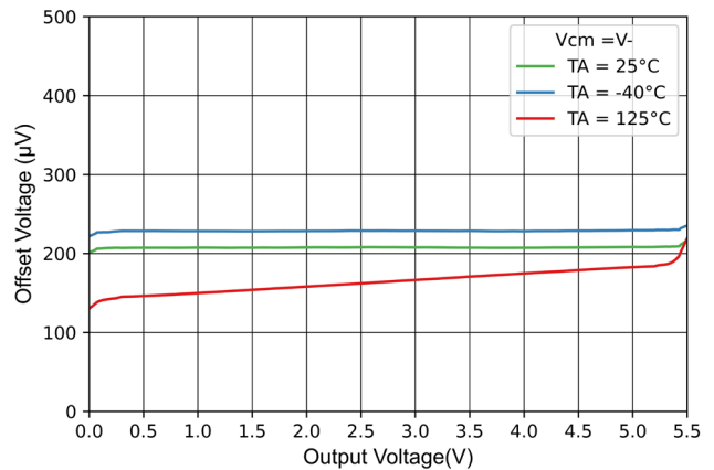
Figure 7-10 Offset Voltage vs Output Voltage
